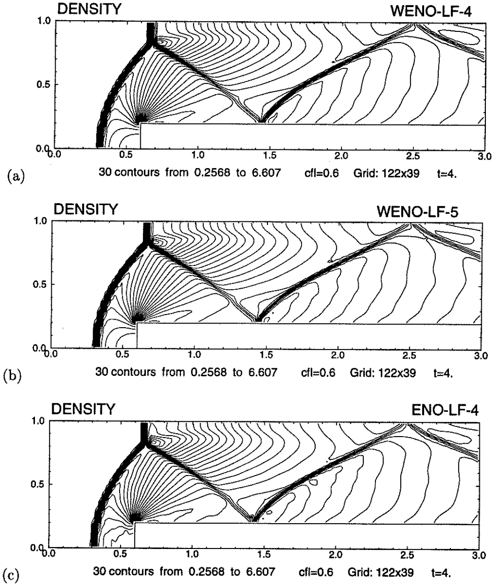
Figure 10: Flow past a forward facing step. Density on medium grid: 122 \times 39 . (a) WENO-LF-4. (b) WENO-LF-5. (c) ENO-LF-4.
