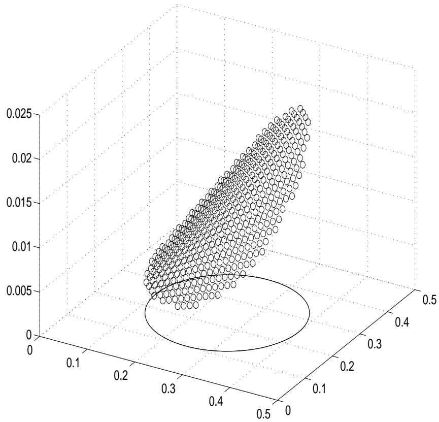
Figure 4: 3D heat equation, T_t = \Delta T , with Dirichlet boundary conditions. The lower dimensional z = .25 cross section of the solution is shown. The circles are the computed solution, and the solid line contour outlines the computational domain.
