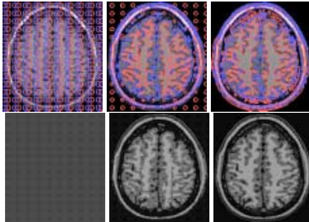
Figure 4.9: Evolution of the four-phase segmentation model from [26], using two level set functions: evolving curves (top) and phases (bottom). The fundamental use of the level-set implementation is once again observed here, since the splitting and merging of the evolving curves is automatically handled, with no programming effort.
