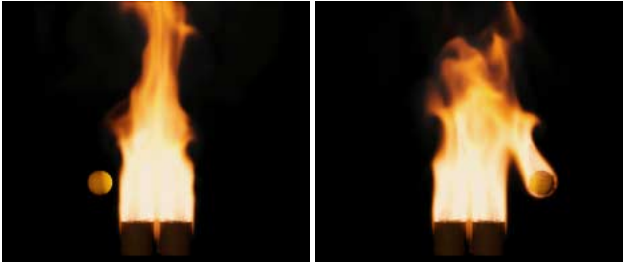
Figure 3.2: The level set method allows one to accurately represent the thin flame zone that separates the unreacted gaseous fuel from the reacted hot gaseous products. This allows one to more accurately model the gaseous expansion across this interfacial zone. Here the level set method is used to simulate a ball catching on fire.
