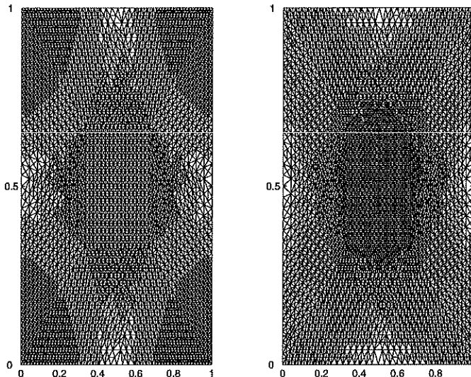
FIGURE 2. The left is the mesh produced by the superconvergence estimator of this paper and the right is the mesh of the residual error estimator of Johnson et al [15, 16]. The L^2 error for the left mesh is 0.0094 with 2279 nodes, and the right mesh has an L^2 error of 0.061 with 2497 nodes.
