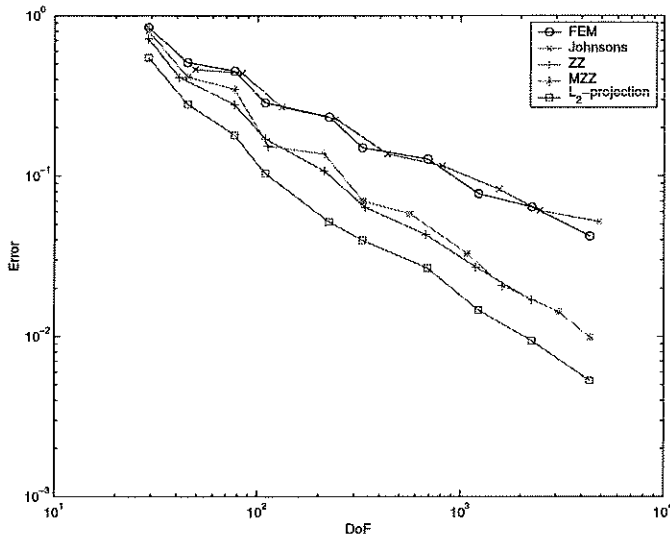
FIGURE 1. Comparison of the mesh quality produced by different recovery methods compared to the error estimator of Johnson et al [15, 16]. All the errors are measured in L^2 for the gradients. FEM refers to the error \|\nabla u_h - \nabla u\|_0 where u_h is the finite element solution over S_h .
