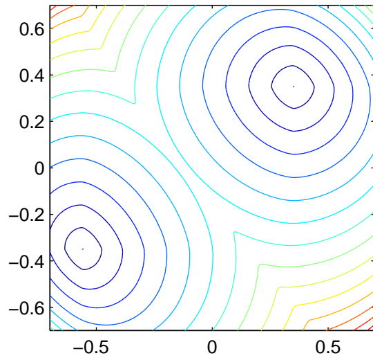
FIGURE 3. This is an example of the distance on a half sphere. The sweeping algorithm applied to the graph of f(x, y) = \sqrt{1.0 - (x^2 + y^2)} with \phi(-0.56, -0.35) = \phi(0.35, 0.35) = 0 as boundary condition on a 100 \times 100 grid. The convergence was reached after 3 sweeping iterations.
