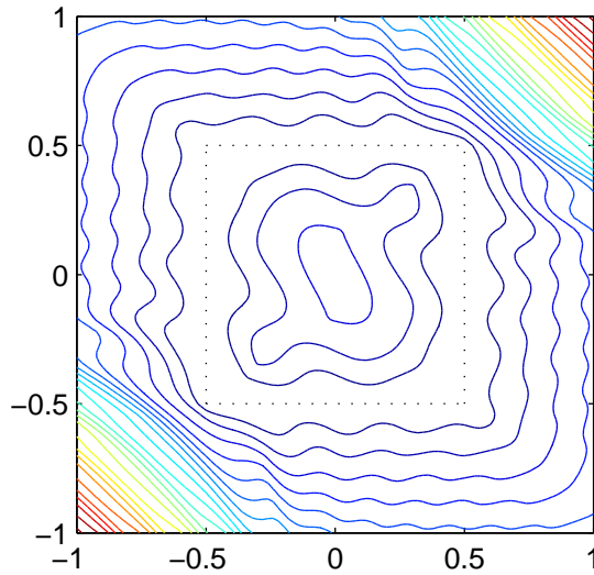
FIGURE 2. (A very degenerate case) a = 0.375 , b = 0.25 , c = 0.29 , and R(x, y) = (2.1 - \cos(4\pi^2 xy))/4.0 on a 100 \times 100 grid. Notice that in this case, ab = 0.0938 is barely greater than c^2 = 0.0841 . Convergence is reached after 45 sweeping iterations.
