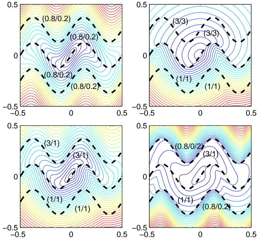
FIGURE 5. This is an example of first arrival travel times in seismic imaging [23]. The computational domain suggests material layering under a sinusoidal profile with layer shapes C(x) = 0.1225 \sin(4\pi x) . Suppose the domain is split into four parts by y_i(x) = 0.1225 \sin(4\pi x) + p_i where i = 1, 2, 3 and p_i = (-0.25, 0, 0.25) . In each layer, the anisotropic speed at (x, y) is given by an ellipse with long axis (of length 2F_2 ) tangential to the curve C(x) and the short axis (of length 2F_1 ) normal to the curve. F_1 and F_2 are constants in each layer. This leads to F_2 \sqrt{((1+n^2)\phi_x^2 + (1+m^2)\phi_y^2 - 2mn\phi_x\phi_y)/(1+m^2+n^2)} = 1 where (m, n) = \frac{\sqrt{(F_2/F_1)^2 - 1}}{\sqrt{1 + (\frac{dC(x)}{dx})^2}} (\frac{dC(x)}{dx}, -1) . The (F_2, F_1) pair for each layer is given in the above figures. The convergence was obtained after 5, 4, 16, and 16 iterations on 200x200 grid.
