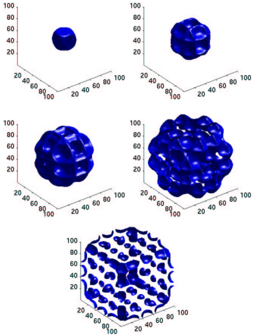
FIGURE 8. This is a 3d example with f(x, y, z) = \cos(2\pi x) \cos(2\pi y) \cos(2\pi z) and the corresponding w = (1 + \nabla f \cdot \theta)^{-1/2} . The convergence was obtained after 10 iterations on 100x100x100 grid. The contours shown here are 1.2, 1.5, 1.8, 2.2, 2.5.
