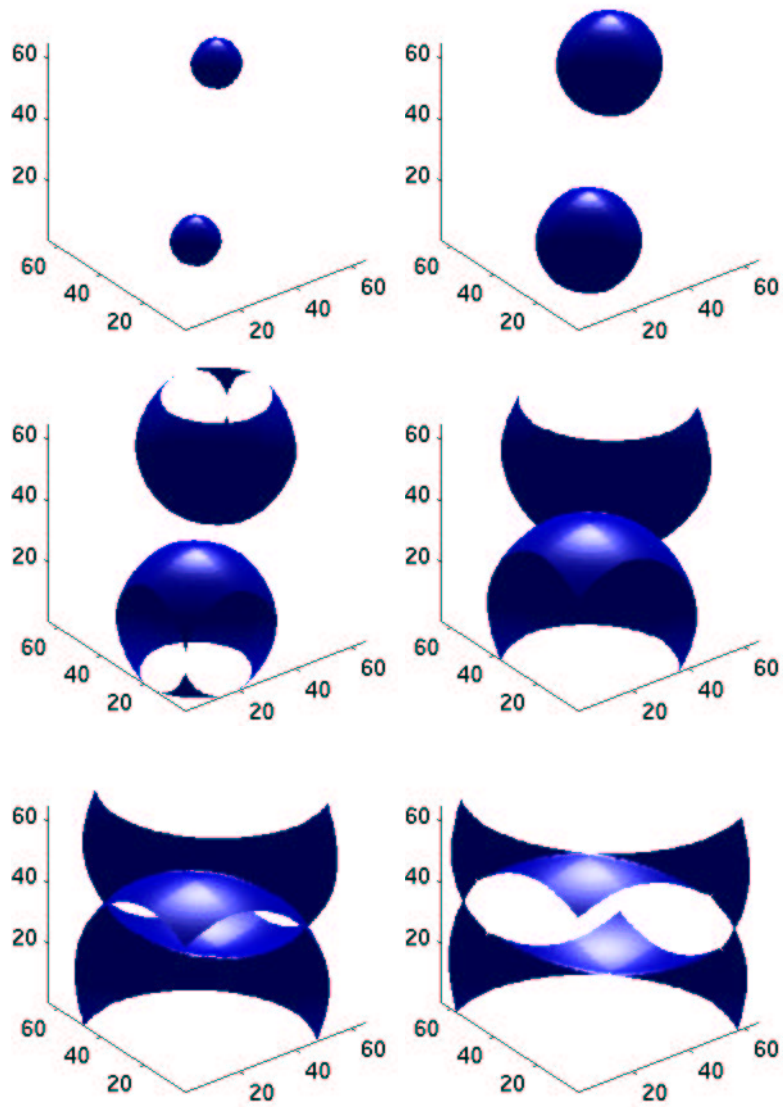
FIGURE 7. This is one-iteration result of the 3D eikonal equation with two boundary points (-0.5, -0.5) and (0.5, 0.5) . The corresponding contours are 0.25, 0.5, 0.75, 1, 1.25, 1.5.
