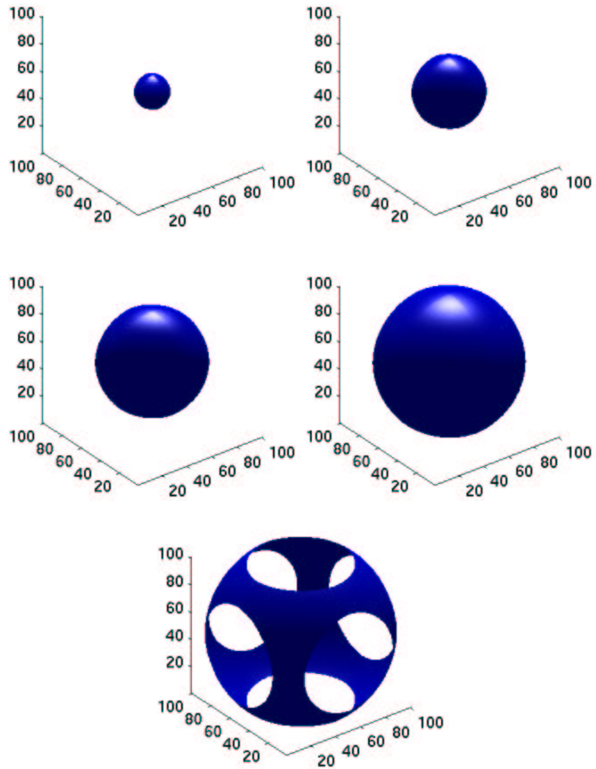
FIGURE 6. This is one-iteration result of the 3D eikonal equation with the boundary (0, 0) in the center of the graph. The corresponding contours are 0.25, 0.5, 0.75, 1.0, 1.25.
