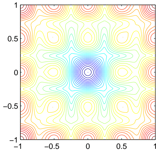
FIGURE 4. The distance contour from (0, 0) on the graph of f(x, y) = \cos(2\pi x) \cos(2\pi y) . The convergence was obtained after 12 iterations on 100 \times 100 grid.
