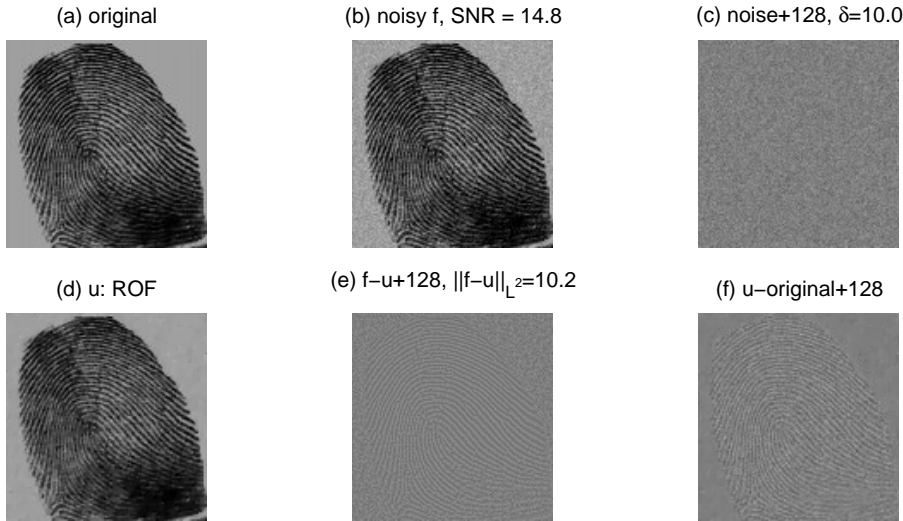
FIGURE 3. ROF with \lambda = 0.085 , \|f - u\|_{L^2} \approx \delta , signal contained in v = f - u .
