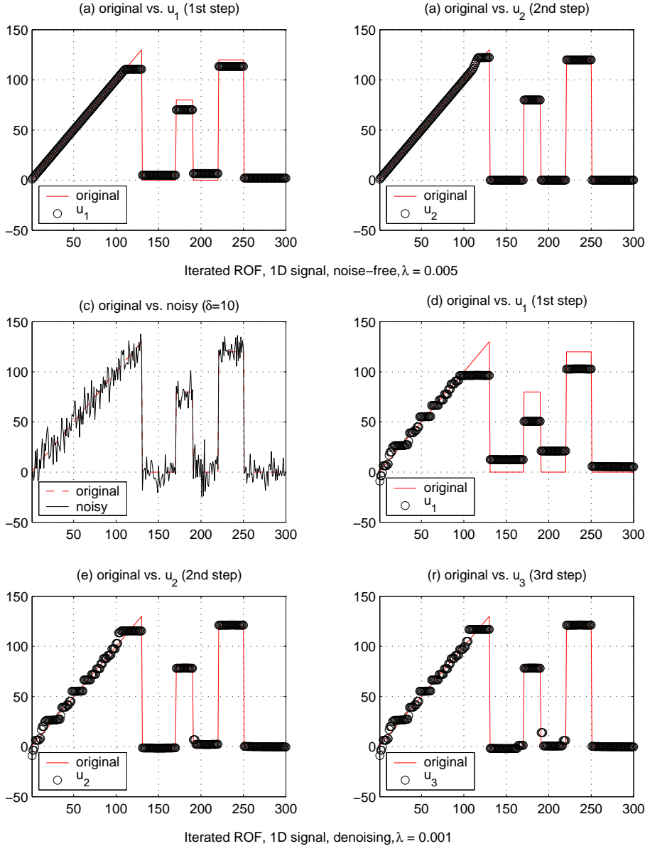
FIGURE 2. ROF and iterative regularization on 1D signal (noise free & noisy) .
