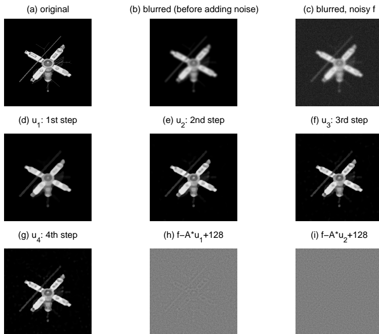
FIGURE 10. ROF with iterative regularization, deblur+denoise, Gaussian blur/noise, \delta = 10 and \lambda = 0.1 .
