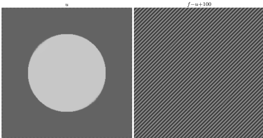
Figure 12: A decomposition using (BV, F) , with v = \operatorname{div}(\vec{g}) with translated dyadic BMO.
