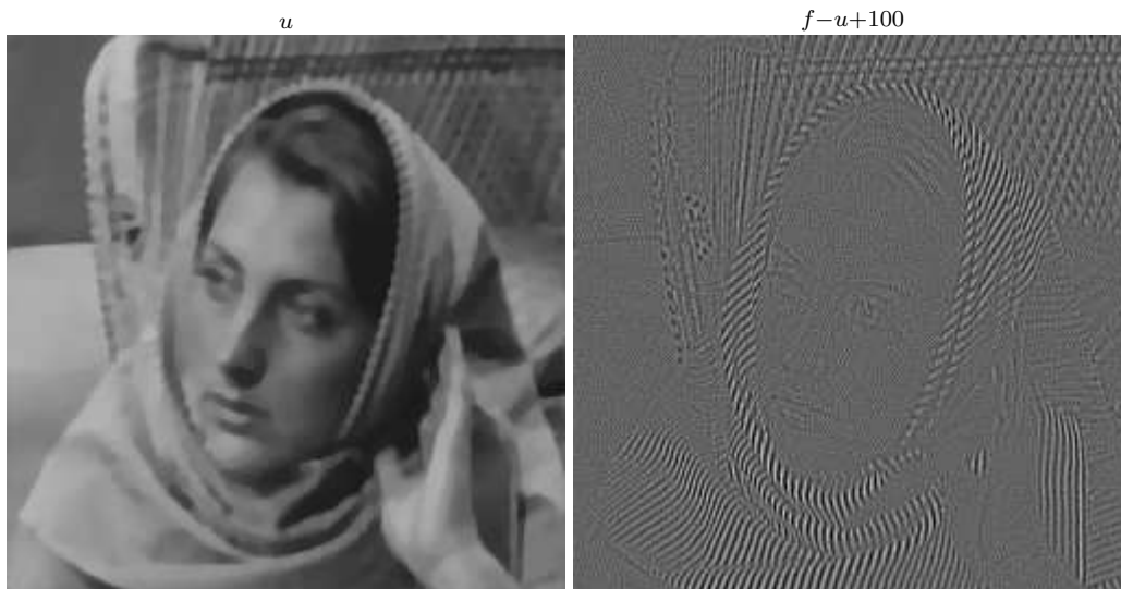
Figure 18: A decomposition using (BV, F) model (40), with v = \Delta P .
