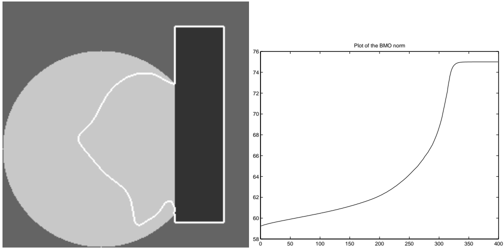
Figure 2: Left: An optimal set which gives \|\cdot\|_{BMO^\beta} . Right: The evolution of the energy (12) versus iterations.
