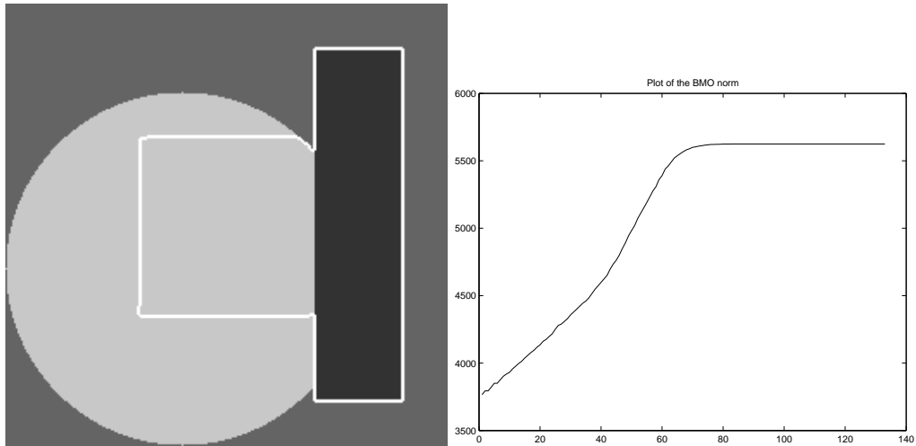
Figure 3: Left: An optimal set which gives \|\cdot\|_{BMO^\beta} . Right: The evolution of the square of the energy (13) versus iterations.
