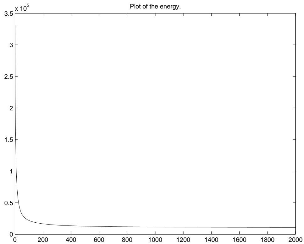
Figure 8: A decomposition using (BV, F) , with v = \text{div}(\vec{g}) , and the plot showing the energy (36) versus iterations. RMSE = 0.0076569 .
