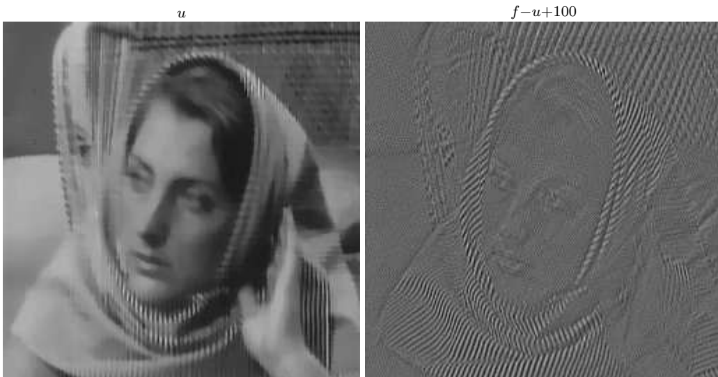
Figure 17: (BV, G) , with v = \text{div}(\vec{g}) decomposition.
