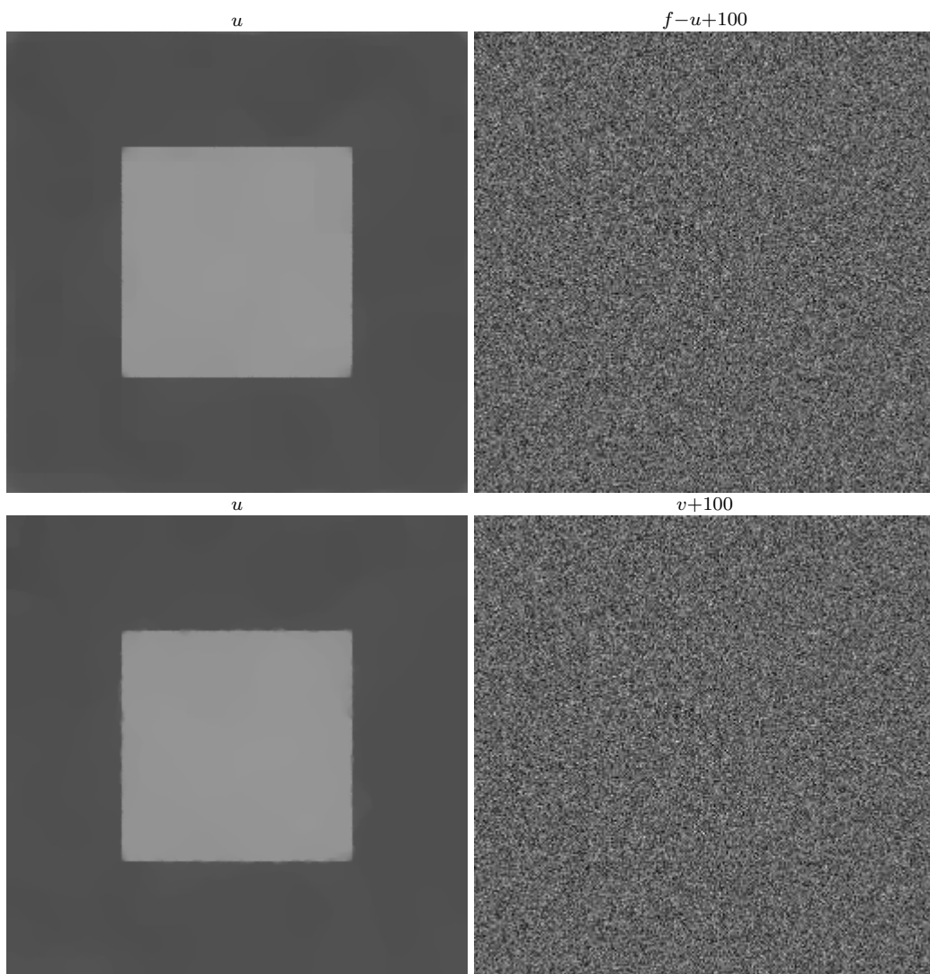
Figure 7: Top: A decomposition using V-O with p = 2 , RMSE = 0.00767165 . Bottom: A decomposition using R-O-F. RMSE = 0.008795368 .
