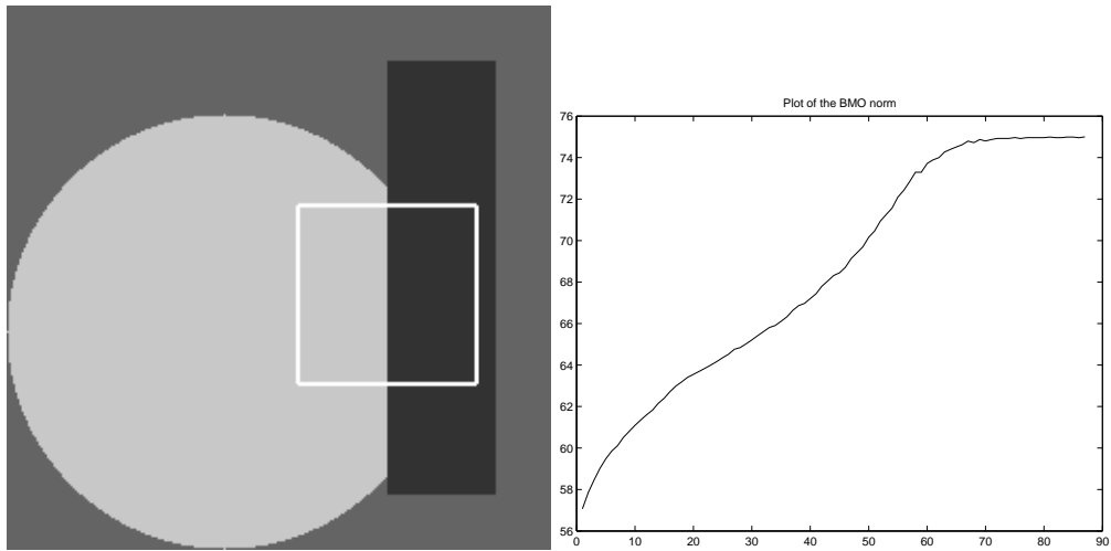
Figure 4: Left: An optimal square which gives \|\cdot\|_{BMO} . Right: The evolution of the energy (14) versus iterations.
