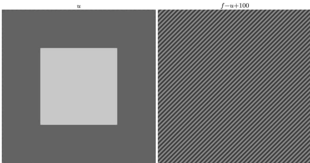
Figure 10: A decomposition using (BV, F) , with v = \operatorname{div}(\vec{g}) with translated dyadic BMO.
