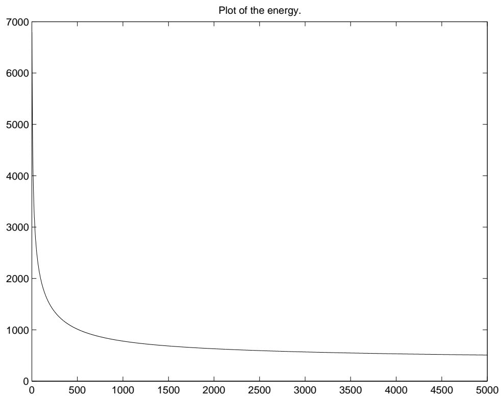
Figure 9: A decomposition using (BV, G) , with v = \text{div}(\vec{g}) , and the plot showing the evolution of the energy (38) (using \|\vec{g}\|_{L^\infty} ) versus iterations. RMSE = 0.00775965 .
