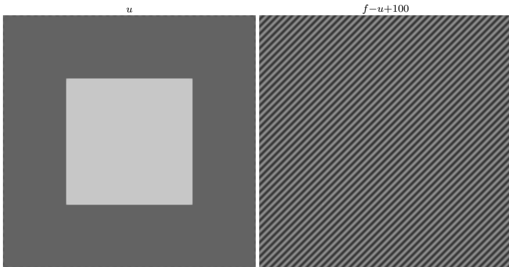
Figure 11: A decomposition using (BV, G) , with v = \operatorname{div}(\vec{g}) .
