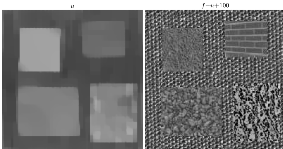
Figure 14: A decomposition using (BV, F) , with v = \text{div}(\vec{g}) .
