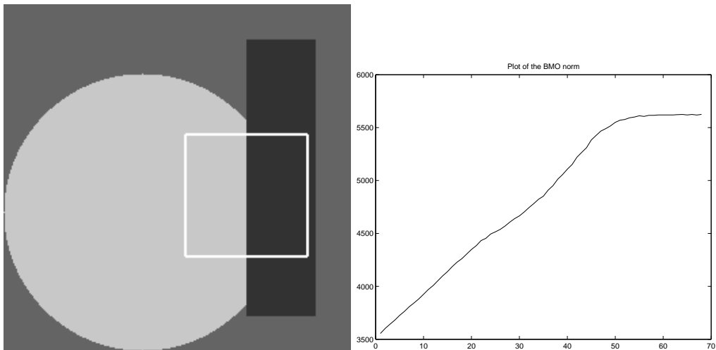
Figure 5: Left: An optimal square which gives \|\cdot\|_{BMO} . Right: The evolution of the square of the energy (15) versus iterations.
