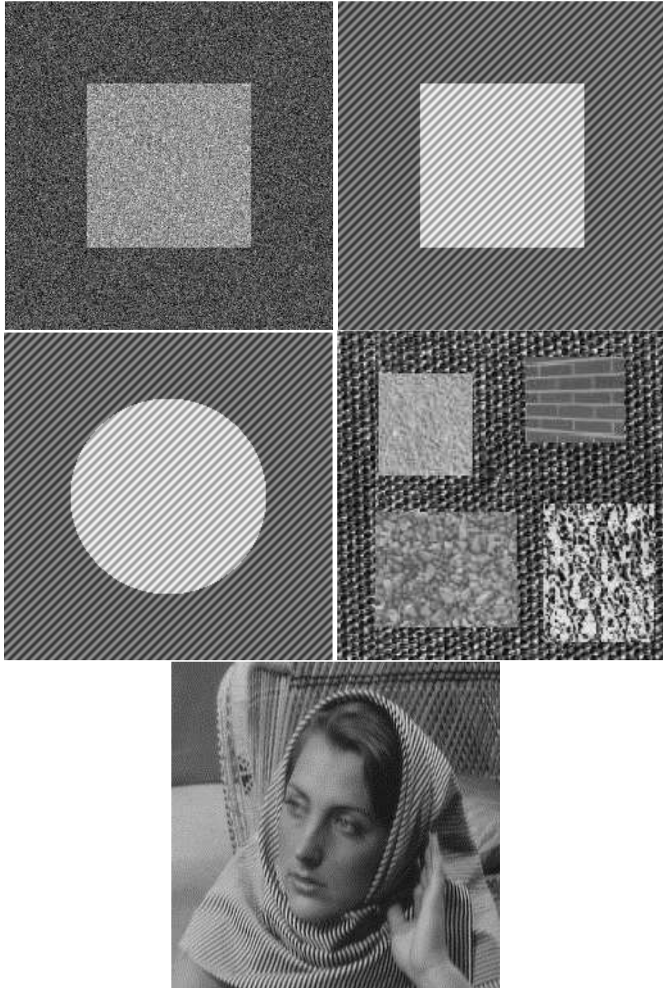
Figure 6: The data images to be decomposed.
