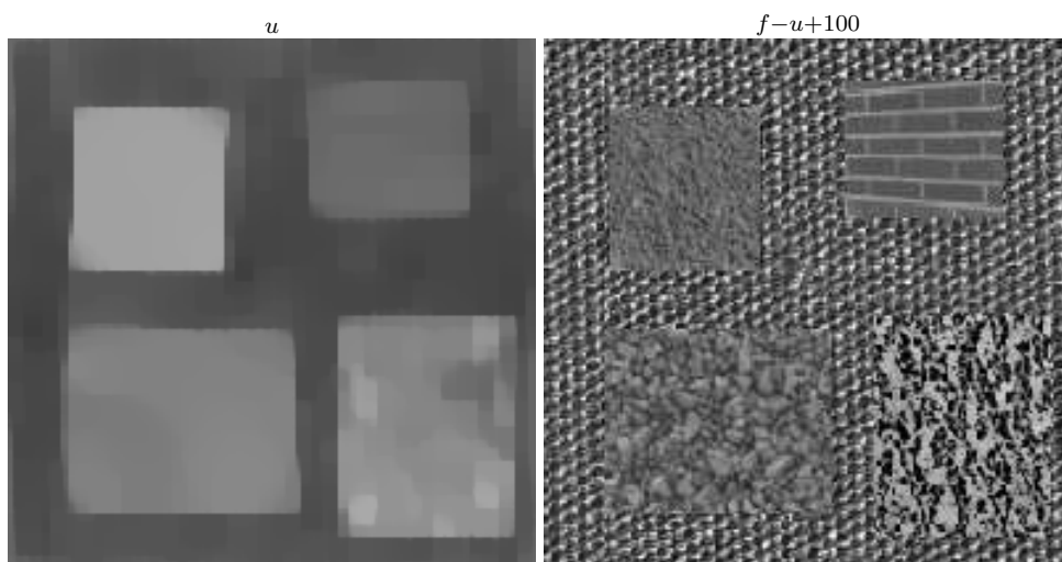
Figure 15: A decomposition using (BV, G) , with v = \text{div}(\vec{g}) .
