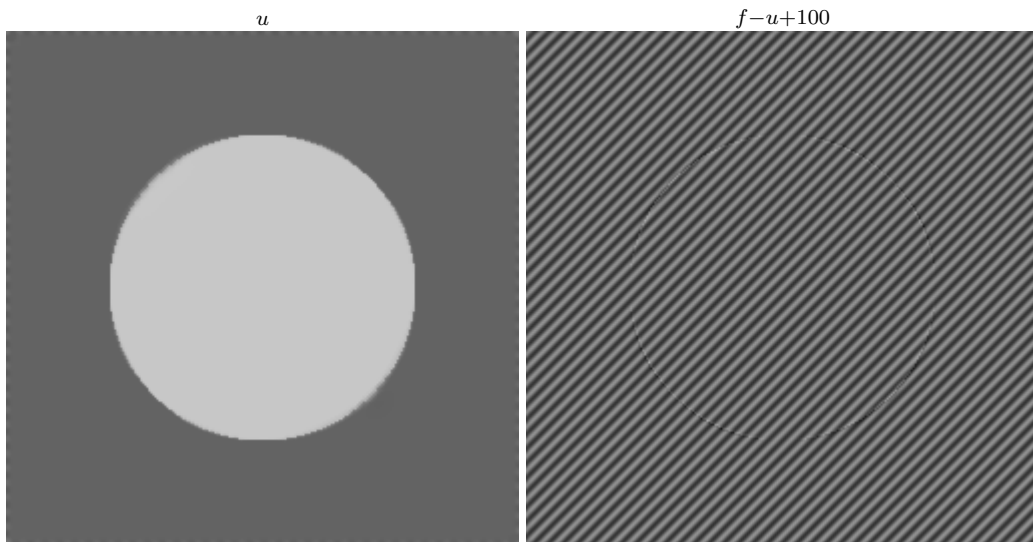
Figure 13: A decomposition using (BV, G) , with v = \operatorname{div}(\vec{g}) .
