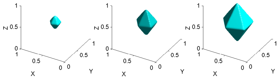
Figure 8: Wulff crystal with surface tension \gamma\left(\frac{\nabla\phi}{|\nabla\phi|}\right) = (1 + 2\sqrt{\sin(|\theta_1| - 0.5\pi)})(1 + |\sin(2.5(\theta_2 + 0.5\pi))|) . Contours from left to right at \phi = 0.08, 0.14, 0.2 .
