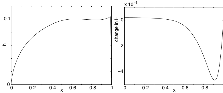
Figure 12: h(x, 7510) and H(x, 7510) - H(x, 7500)
