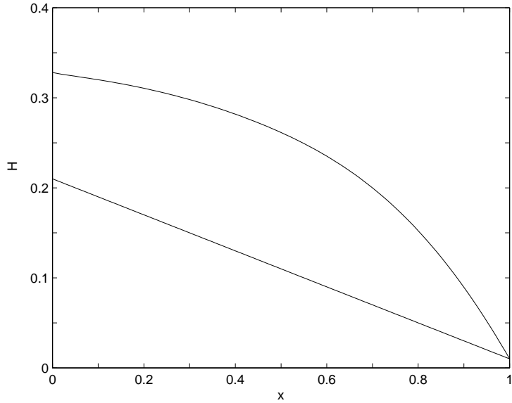
Figure 9: H(x, 7500) (curved) and H(x, 0) (linear)
