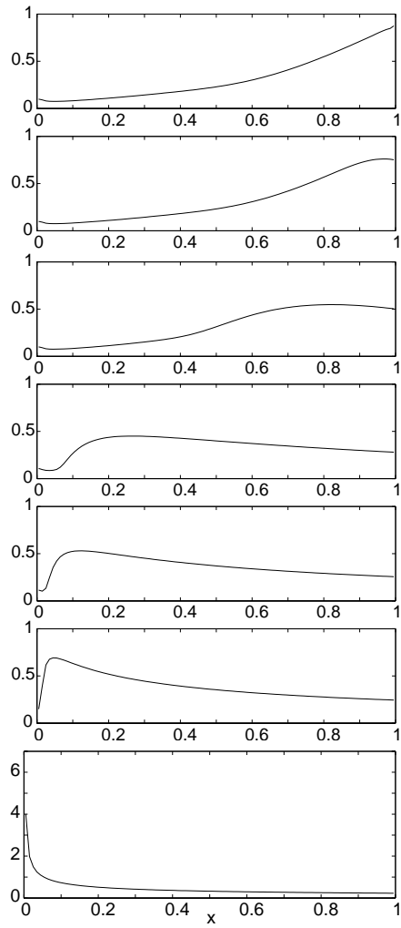
Figure 16: S(x,t) = -H_x for 7500 \leq t \leq 16000
