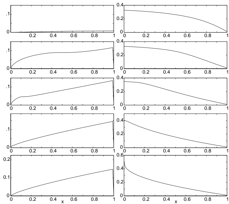
Figure 15: h(x,t) and H(x,t) for 7500 \leq t \leq 16000
