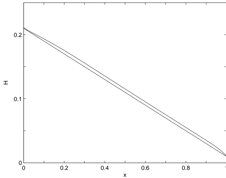
Figure 8: H(x, 250) (curved) and H(x, 0) (linear)
