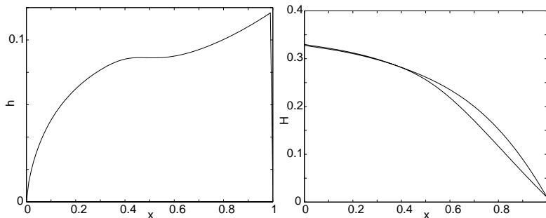
Figure 14: h(x, 7600) ; and H(x, 7600) with H(x, 7500)
