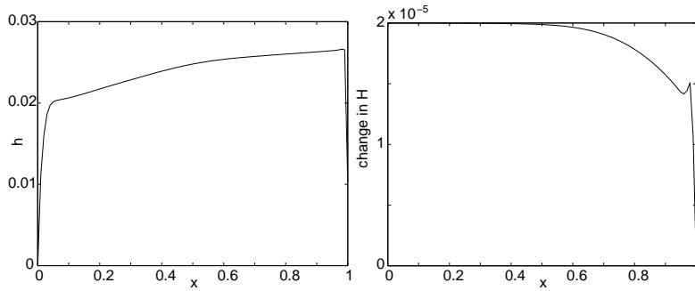
Figure 11: h(x, 7501) and H(x, 7501) - H(x, 7500)
