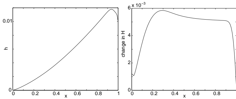
Figure 7: h_{\text{old}}(x, 250) and H(x, 250) - H(x, 0)
