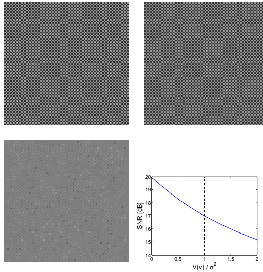
Fig. 4. Approaching worst-case scenario in a checkered-board image. For V(v) = \sigma^2 , the SNR decreases by almost 3dB from 19.9dB to 17.0dB . Top: f (left), u (right). Bottom: v (left), SNR as a function of V(v)/\sigma^2 (right).
