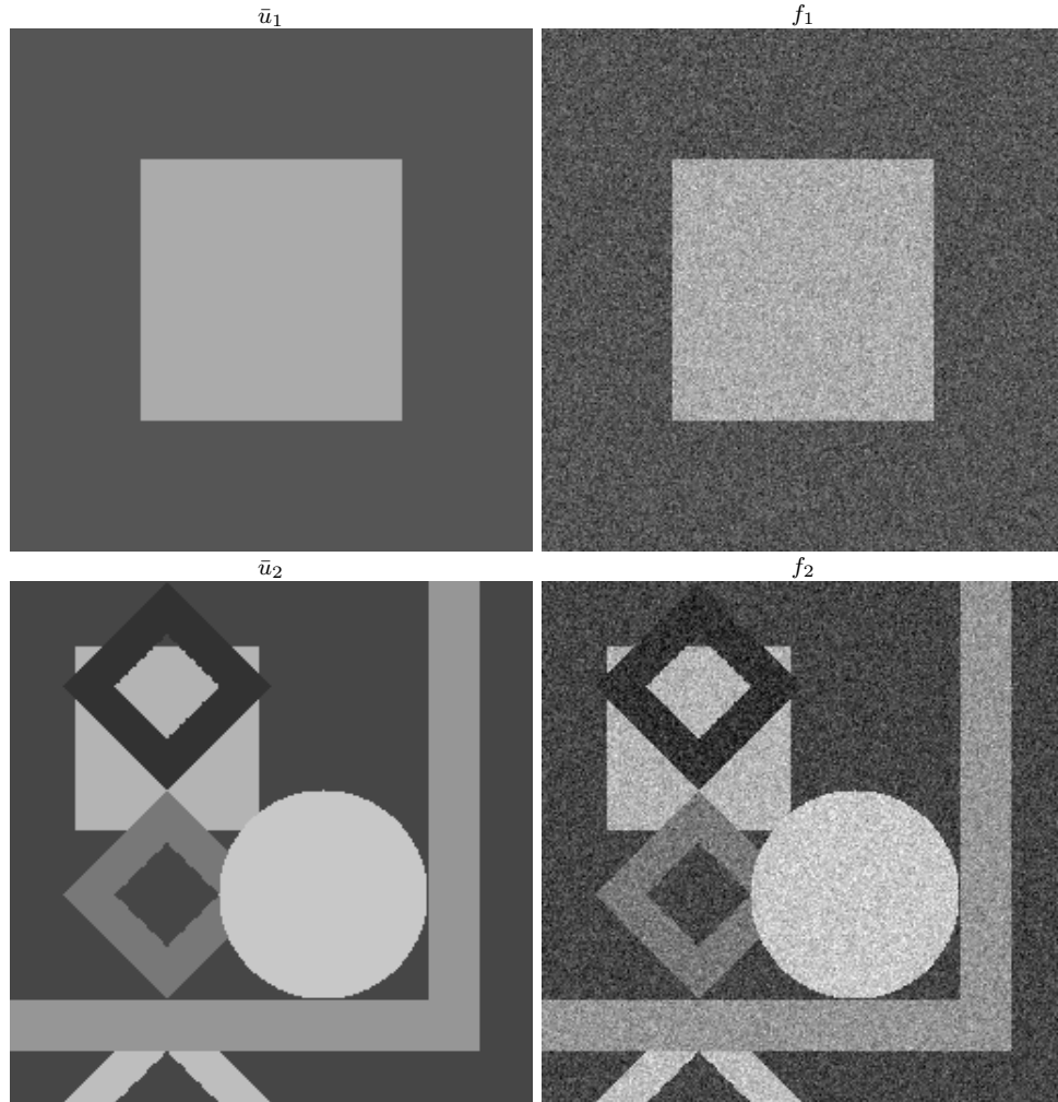
Figure 18: Exact cartoon images and their noisy versions corrupted by additive Gaussian noise
