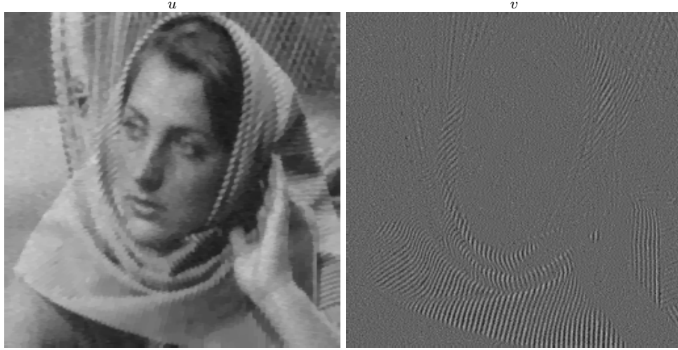
Figure 23: A decomposition of the noisy image f_2 from Figure 2 using the model (59) with the kernel being the characteristic function of a square centered at 0 having 3-pixel length for the sides, \varphi(\nabla u) = |\nabla u| , p = 1 , and \lambda = 2 .
