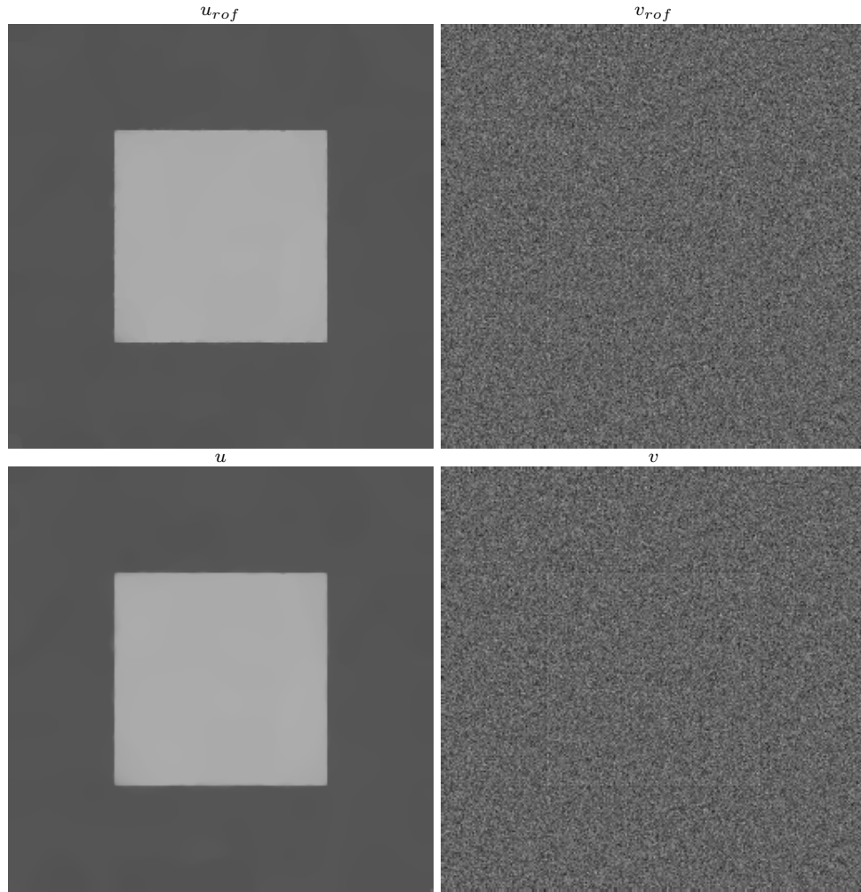
Figure 19: The top row shows a decomposition of f_1 from Figure 18 using the R-O-F model (2) with rmse = 1.3923 . The bottom row shows a decomposition of the same image using W_t , p = 2 and \alpha = 1 in (50) with rmse = 1.7200 .
