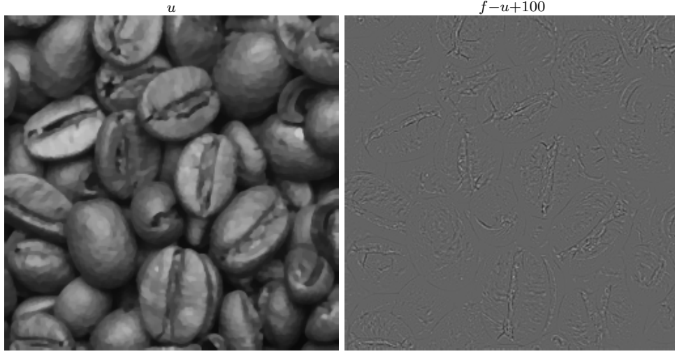
Figure 14: A decomposition of f_3 using P_t in (50) with \varphi(\nabla u) = |\nabla u| , \alpha = 1 , p = 1 , \lambda = 1500 .
