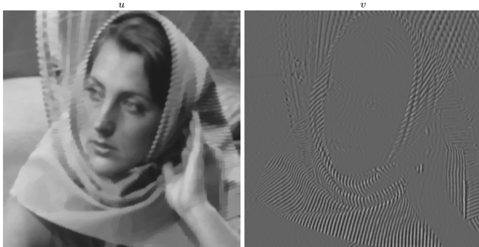
Figure 22: A decomposition of f_1 from Figure 2 using the model (59) with the kernel being the characteristic function of a square centered at 0 having 5-pixel length for the sides, \varphi(\nabla u) = |\nabla u| , p = 1 , and \lambda = 1.5 .
