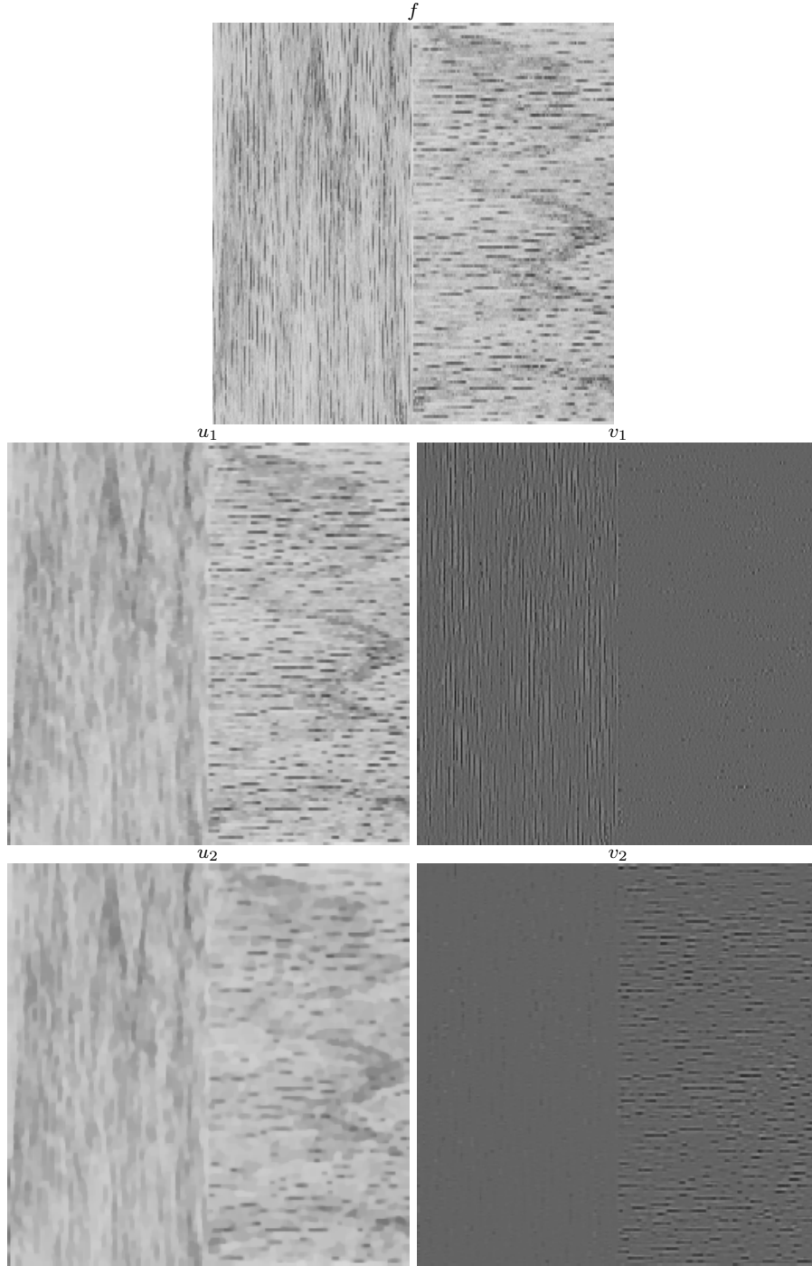
Figure 26: (u_1, v_1) is a decomposition of f = u_1 + v_1 using the model (59) with the kernel being the characteristic function of a horizontal line centered at 0 having 3-pixel length. u_1 is then decomposed into u_2 + v_2 using the same model with the kernel being the characteristic function of a vertical line centered at 0 having 3-pixel length. The two decompositions have \varphi(\nabla u) = |\nabla u| , p = 1 , and \lambda = 2 .
