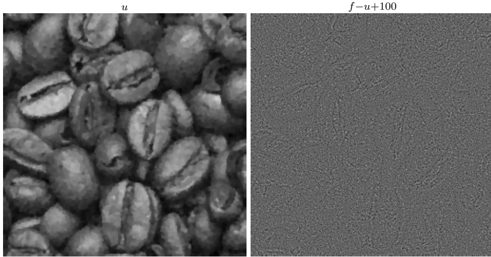
Figure 15: A decomposition of the noisy image f_4 using P_t in (50) with \varphi(\nabla u) = -\beta + \sqrt{|\nabla u|^2 + \beta^2} , \beta = \sqrt{10} , \alpha = 1 , p = 1 , \lambda = 1500 .
