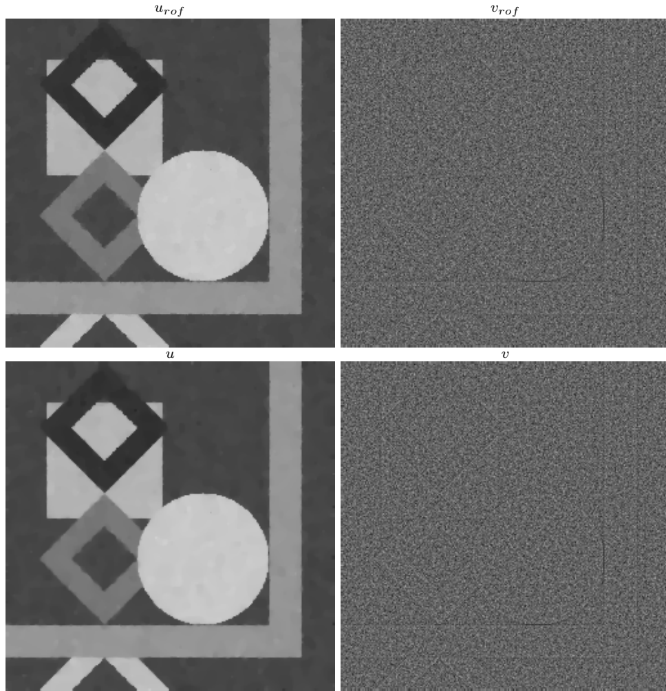
Figure 20: The top row shows a decomposition of f_2 from Figure 18 using the R-O-F model (2) with rmse = 4.4287 . The bottom row shows a decomposition of the same image using W_t , p = 2 and \alpha = 1 in (50) with rmse = 4.7221 .
