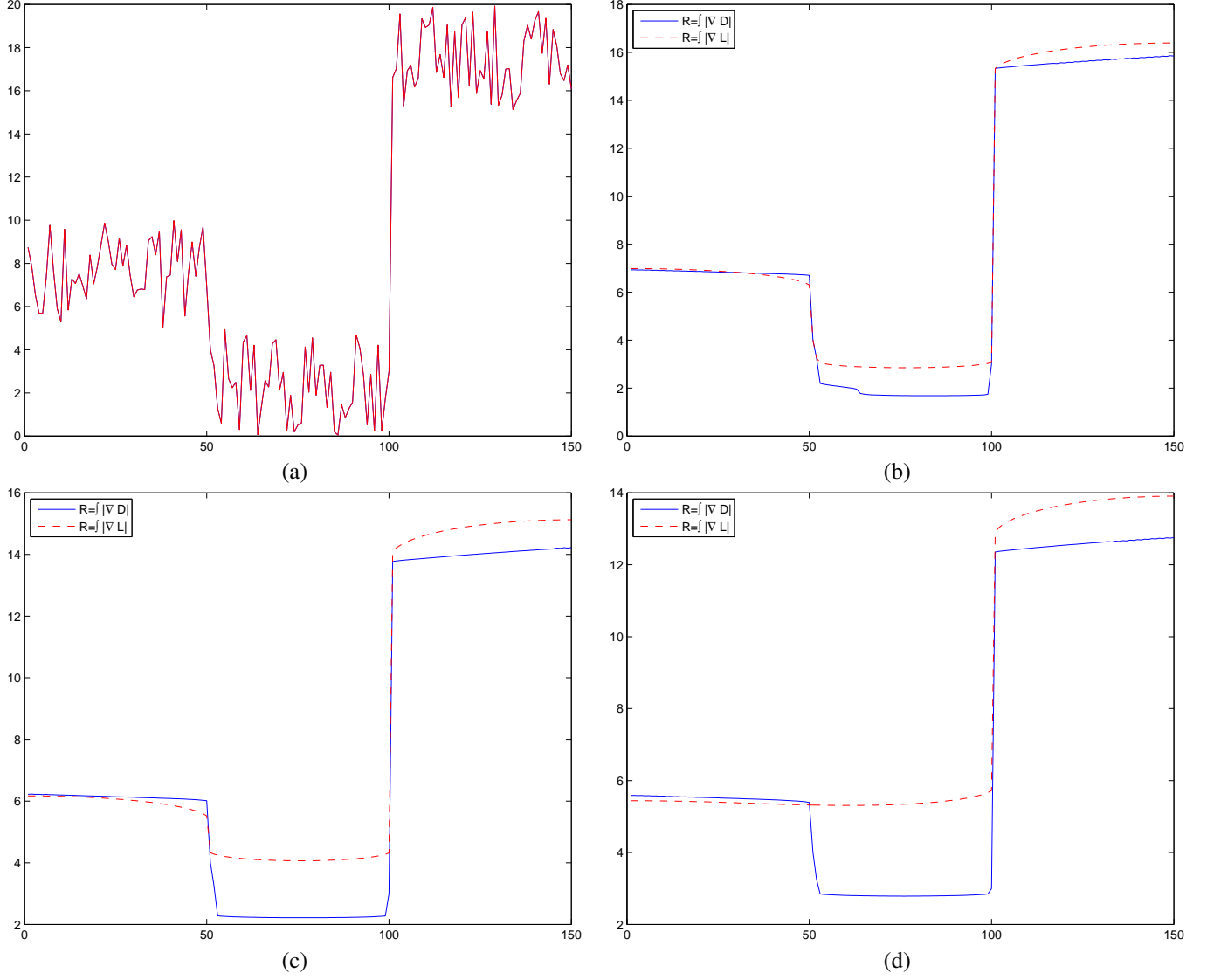
Fig. 3. A simple 1D example showing the qualitative behavior of the model for regularizers \int_{\Omega} |\nabla L| and \int_{\Omega} |\nabla D| . The noisy signal in (a) is processed with both flows. Figures (b), (c) and (d) are snapshots during the flow at the three times t = 8 , t = 16 and t = 24 .
