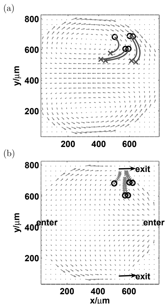
Fig. 8 The displacement of particles starting at random positions denoted by \text{O} s. (a) The instantaneous velocity field at t_w = 150 \text{ ms} and z = 148 \mu\text{m} . \text{X} s denote the particle positions after 150 ms of convection by the instantaneous velocity field; (b) The overall displacement field at z = 148 \mu\text{m} by the forward-and-back droplet actuations. The flow enters the z plane near the nose and the tail of the droplet and exits out of the plane near the front half of the meniscus. \text{X} s denote the ending positions of each cycle.
