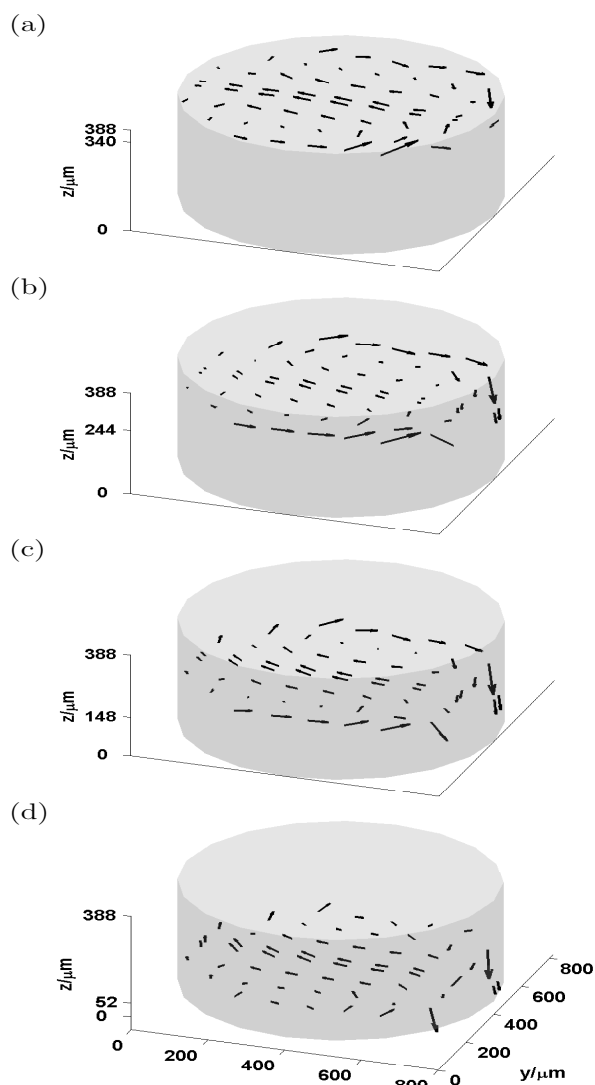
Fig. 6 The 3-dimensional velocity field at (a) z = 340 \mu\text{m} ; (b) z = 244 \mu\text{m} ; (c) z = 148 \mu\text{m} ; (d) z = 52 \mu\text{m} .
