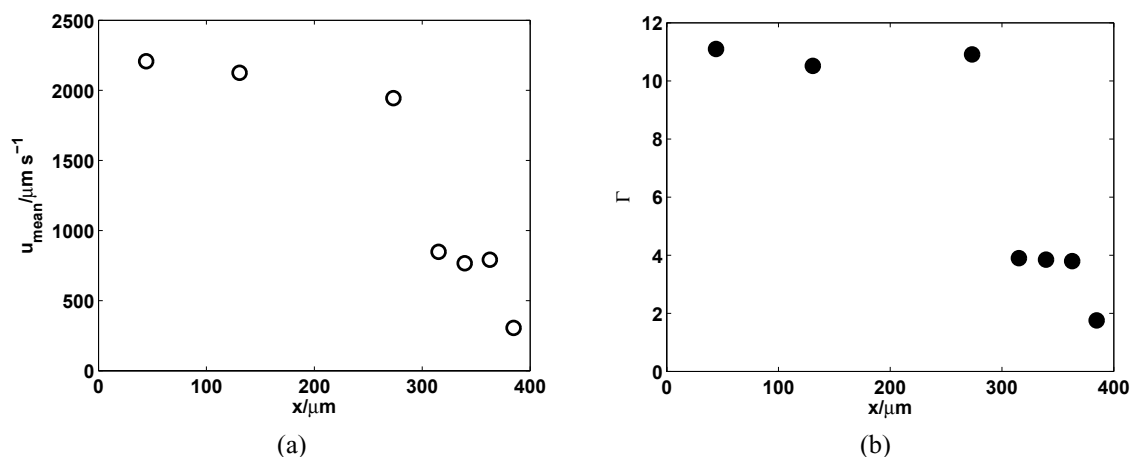
Fig. 5 (a) Mean velocity of the droplet at different locations; (b) Circulation strength of the flow at different center of masses locations.
