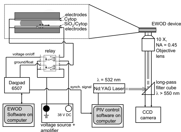
Fig. 1 EWOD device and PIV experimental setups.
