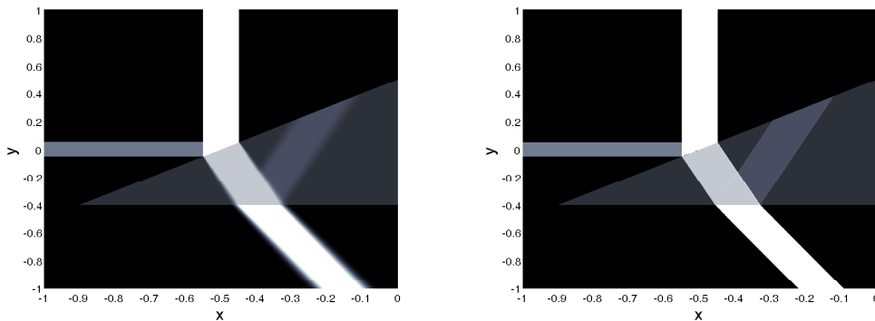
Figure 12: Example 5.4, a bird's eye view of the density with interface plotted, to better illustrate the result, density was taken to be 2.5 times the original one. Left: numerical solution. Right: true solution.
