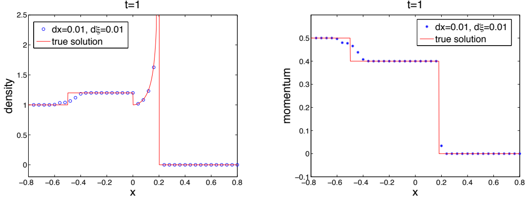
Figure 3: Example 5.3, the comparison of density and momentum between the reference solution and numerical solution at t=1 .
