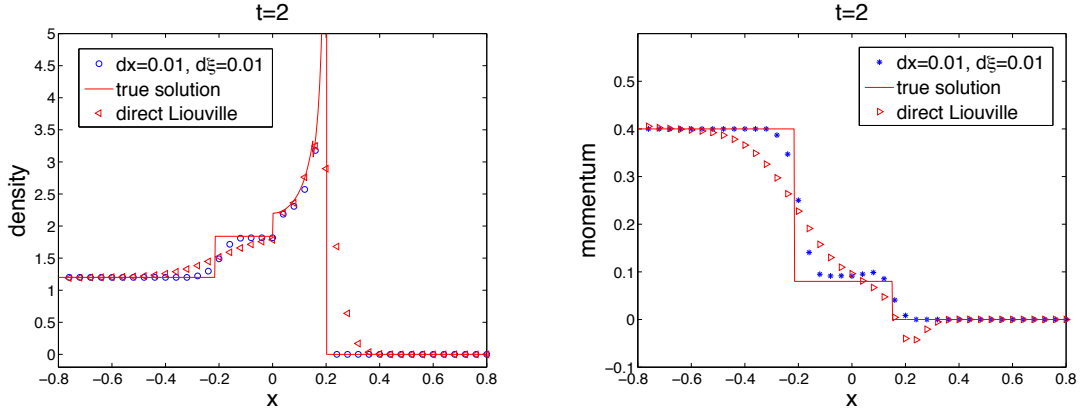
Figure 7: Example 5.3, the comparison of density and momentum between the solutions obtained by our method and by the direct method.
