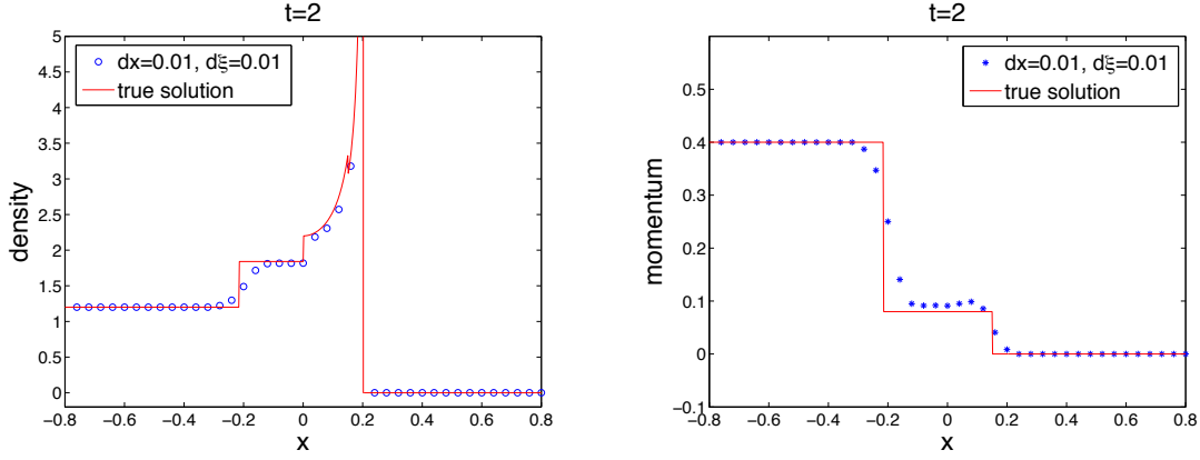
Figure 4: Example 5.3, the comparison of density and momentum between the reference solution and numerical solution at t=2 , reinitialization was performed at t=1 .
