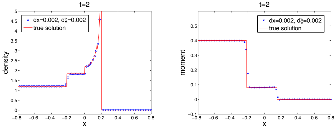
Figure 5: Example 5.3, the comparison of density and momentum between the reference solution and numerical solution at t=2 with a finer grid and b = 0.15\sqrt{\Delta x} , reinitialization was performed at t=1 .
