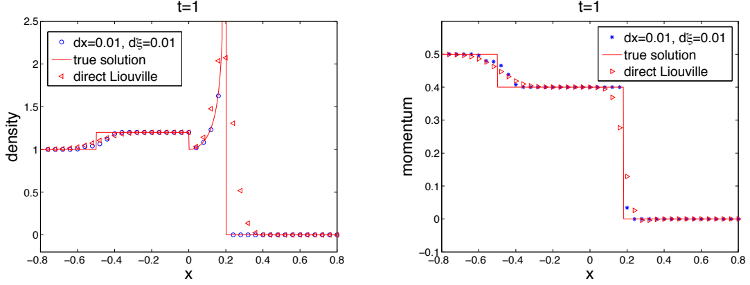
Figure 6: Example 5.3, the comparison of density and momentum between the solutions obtained by our method and by the direct method.
