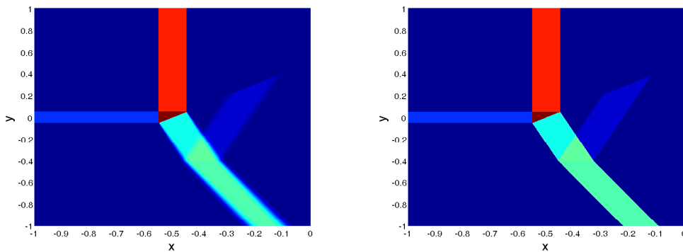
Figure 11: Example 5.4, a bird's eye view of the density. Left: numerical solution. Right: true solution.
