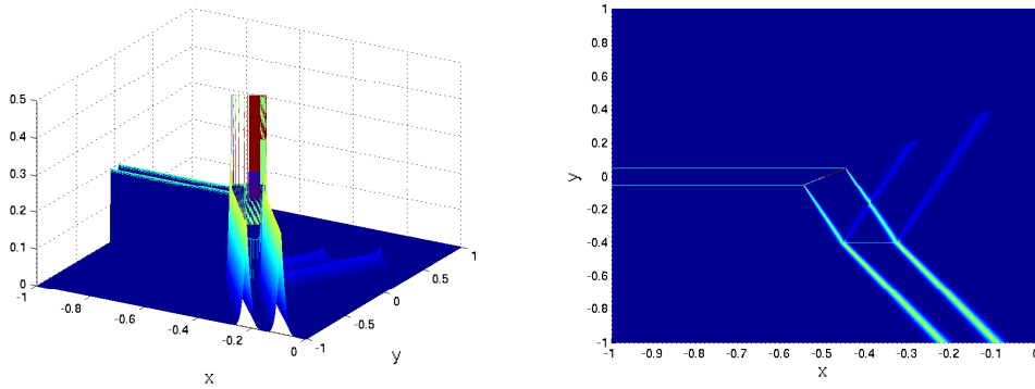
Figure 10: Example 5.4, the difference between the numerical solution and true solution at t=1 (left), a bird's eye view of the difference (right).
