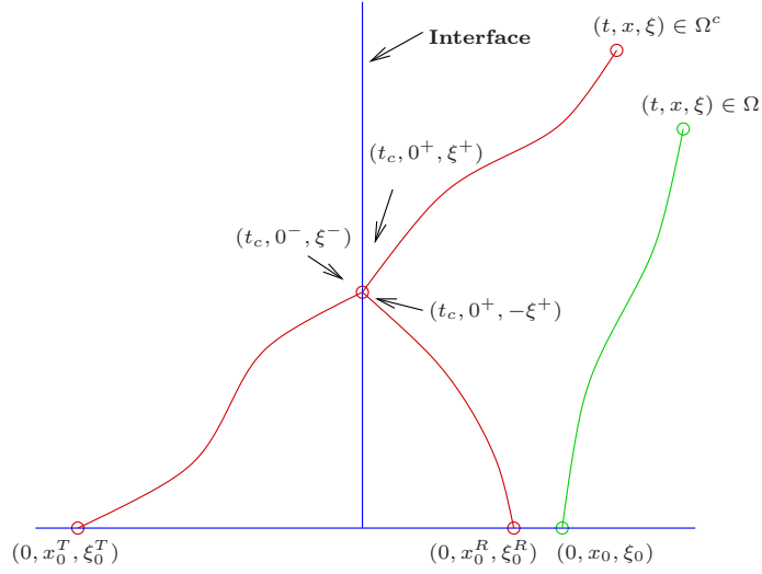
Figure 1: Illustration of the characteristic solution.
