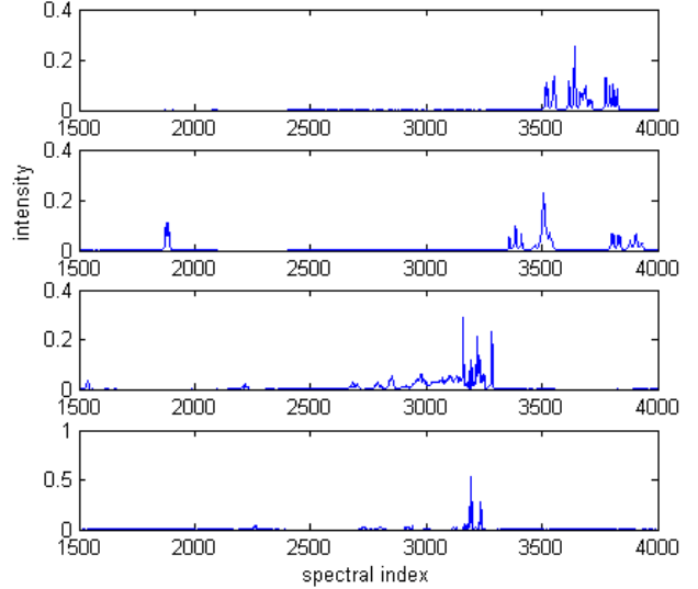
Fig. 8: Four NMR source spectra from [1] Fig. 4
