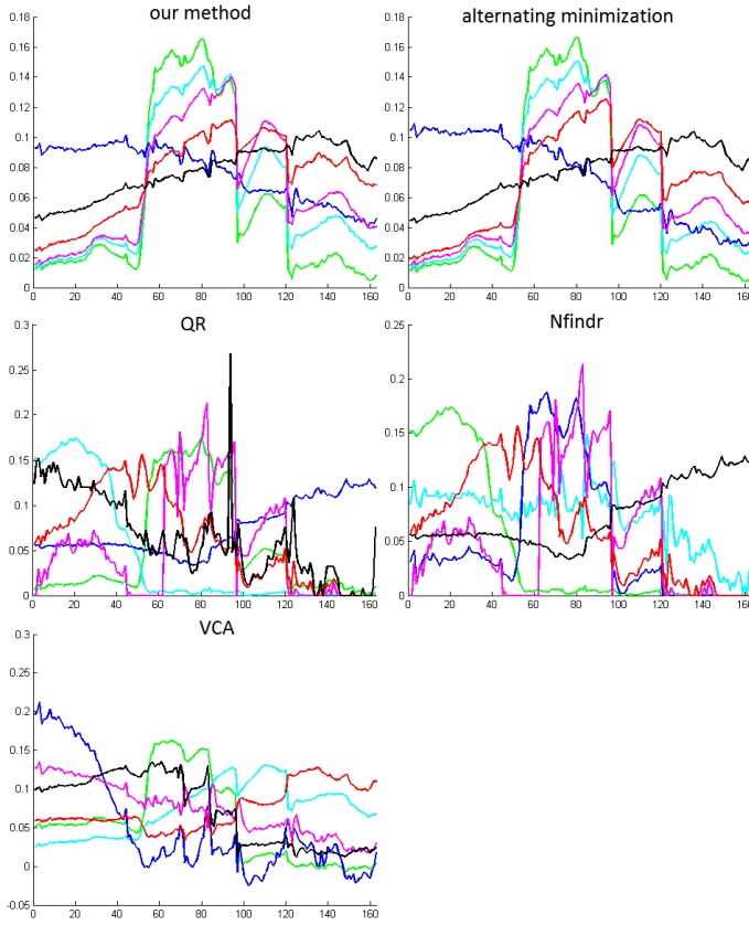
Fig. 4: Spectral signatures of endmembers extracted by different methods.
