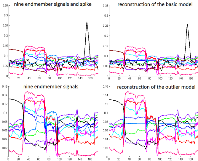
Fig. 7: Comparison between the basic and the outlier method on Indian pines data with outliers
