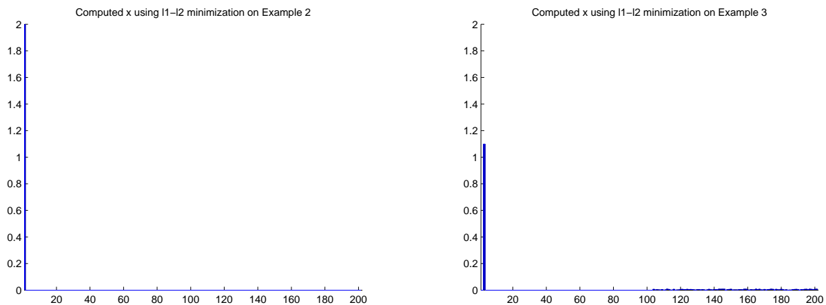
Fig. 4. Estimated x using Algorithm 3 on (4.5).
