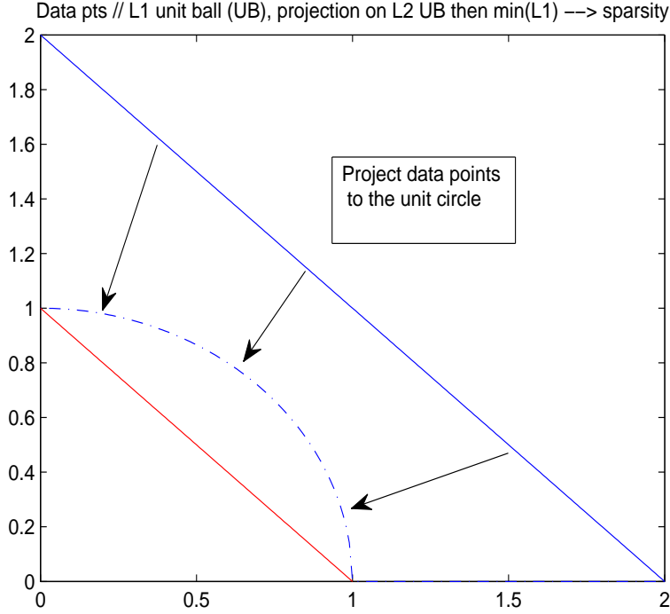
Fig. 1. Illustration of the advantage of minimizing \frac{l_1}{l_2} over l_1 when data points (on x_1 + x_2 = 2 in the first quadrant) lie parallel to the l_1 unit ball. Minimization of \frac{l_1}{l_2} is same as projection onto the unit l_2 ball then intersecting with the unit l_1 ball to select sparse solutions. In contrast, l_1 minimization cannot distinguish sparse data points.
