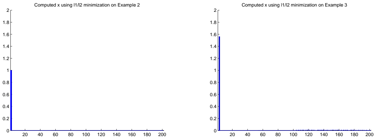
Fig. 3. Estimated x using Algorithm 1 on (4.5).
