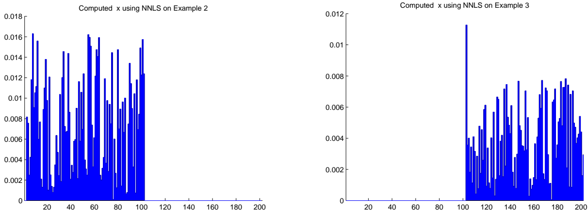
Fig. 2. Estimated x using non-negative least squares.
