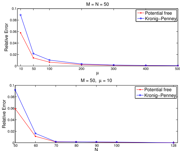
Fig. 6. Relative eigenvalue error of the 1D free-electron model (red dots) and 1D KP model (blue circles). Top: relation of the relative error via different values of \mu for fixed M = N = 50 . Bottom: relation of the relative error via different values of N for fixed \mu = 10 and M = 50 .
