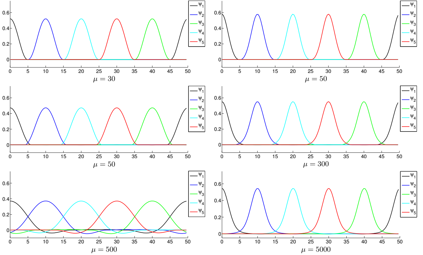
Fig. 4. Computation results of CMs with different values of \mu . The first column: the first 5 CMs of the 1D free-electron model. The second column: the first 5 CMs of the 1D Kronig-Penny model.
