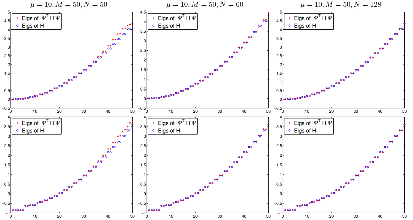
Fig. 5. Comparisons of the first 50 eigenvalues of the 1D free electron model (the first row) and the 1D Kronig-Penney model (the second row).
