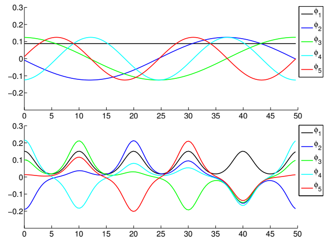
Fig. 3. The first 5 eigenfunctions of the Schrödinger operator \hat{H} in the free-electron model (top) and the KP model (bottom).
