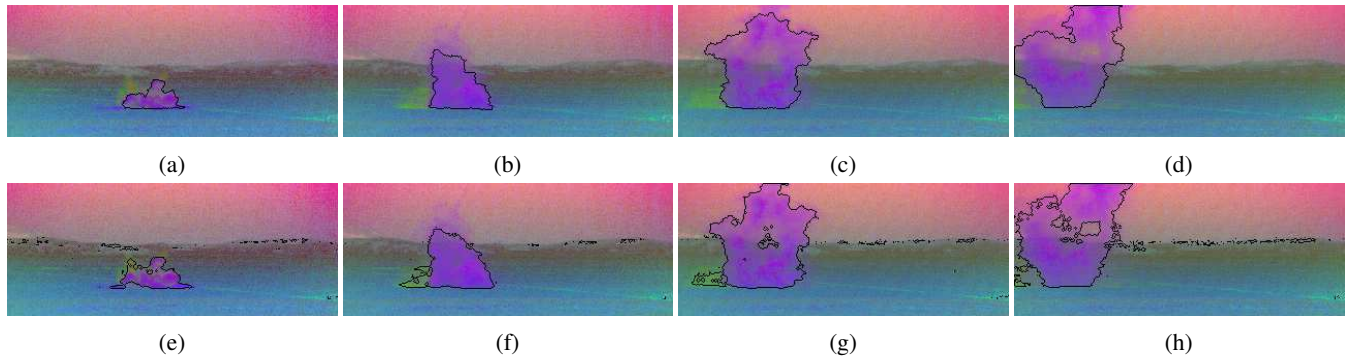
Fig. 5: Top row: segmentation results obtained by the presented method for four frames of the video sequence. Bottom row: segmentation results obtained by [5] for the same frames. Results are displayed on the false color representation video sequence.
