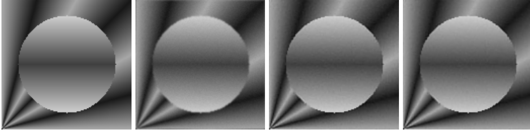
Figure 1: From left to right, the original image, the blurry and noisy, and the deblurring images using the analysis based model (1.5) with a = 0.2 and the general model (4.1) with q = 1 , \nu_1 = 0.2 , \nu_2 = 0.2 . The PSNR values of the recovered images from the analysis based model and the general model are 37.9372 and 38.5268 respectively.
