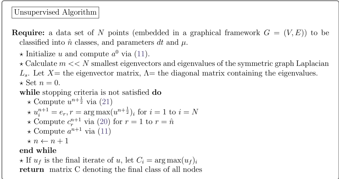
Figure 2: Unsupervised Algorithm
