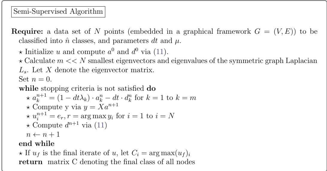
Figure 1: Semi-Supervised Algorithm
