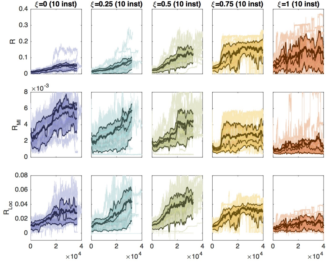
Figure 11: Experimental results on Svenja. Here we set r_{\text{MI},t} equal to the average of the mutual information per entire leg, scaled to have a maximum possible value of 0.1, two bits per continuous degree of freedom, and optimized the time average of r_t = \text{sign}(r_{\text{Loc},t}) \cdot |r_{\text{Loc},t}|^\xi \cdot r_{\text{MI},t}^{1-\xi} . The other details are as in Figure 5.
