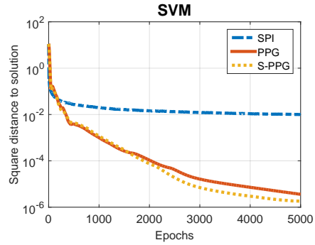
Figure 5: Convergence of SVM example.
