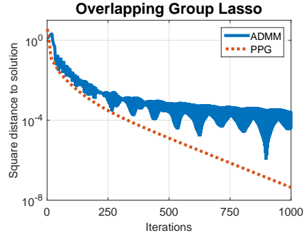
Figure 4: Convergence of overlapping group lasso example.
