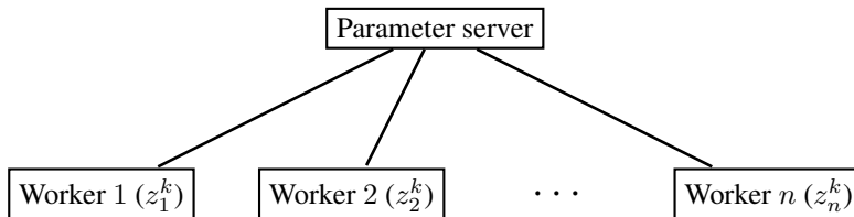
Figure 1: When (PPG) is implemented on a parameter server computing model, the worker nodes communicate (synchronously) with the parameter server but not directly with each other.
