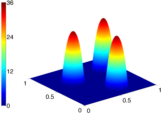
Fig. 2. A domain with three blob functions G_\delta(\mathbf{x}) , where \delta = 0.15 .
