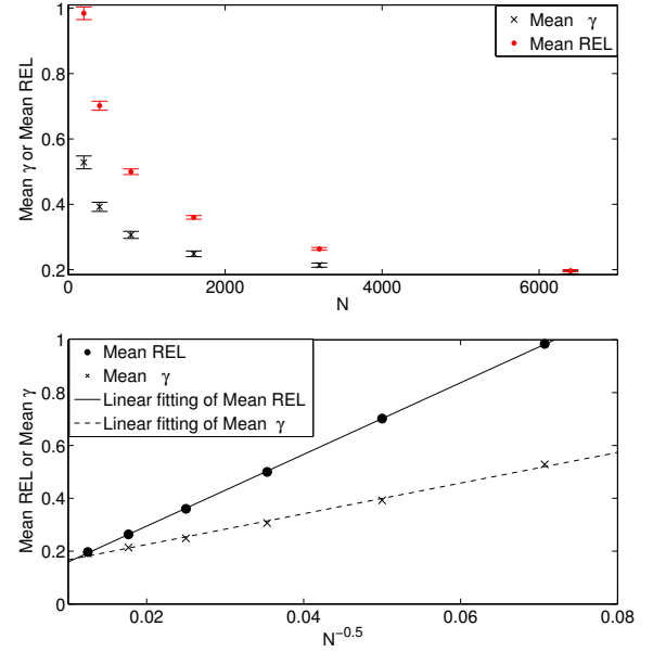
Fig. 5. Top figure: Swarm size N vs. mean REL and mean \gamma , both averaged over 100 simulations of the microscopic model for each value of N . The corresponding standard deviations are shown as error bars. Bottom figure: 1/\sqrt{N} vs. mean REL and mean \gamma . The solid and dashed lines are the linear fittings of mean REL and mean \gamma , respectively.
