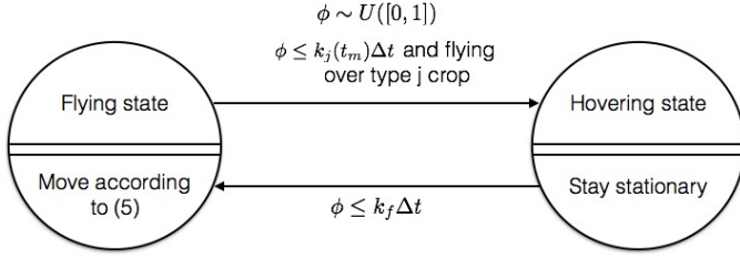
Fig. 1. State-transition diagram of robot controller for pollination. The diagram outlines a program that would run on a single robot.
