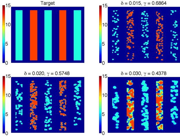
Fig. 7. Top left: Target pollination distribution \rho_\Omega(\mathbf{x}) . From top right to bottom right: Actual pollination distribution \rho_3^{\delta}(\mathbf{x}, T) from the microscopic model with N = 100 robots and \delta = 0.015, 0.020, 0.030 . The discrepancy \gamma is shown for each value of \delta . The field is [0, 1]^2 .
