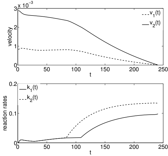
Fig. 3. Top : robot velocity field \mathbf{v}(t) = (v_1(t), v_2(t)) . Bottom : robot pollination rates k_1(t) and k_2(t) .
