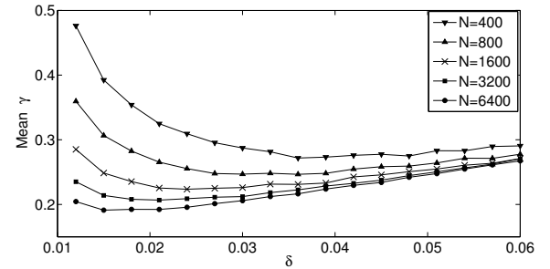
Fig. 6. Relationship among \delta , N , and \gamma . Each data point is averaged over 100 simulations of the microscopic model with the corresponding values of N and \delta .
