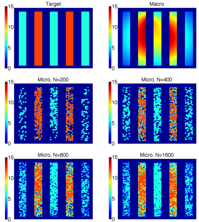
Fig. 4. Top left : Target pollination distribution \rho_\Omega(\mathbf{x}) . Top right : Expected pollination distribution \rho_3(\mathbf{x}, T) from the macroscopic model. From middle left to bottom right : Actual pollination distribution \rho_3^\delta(\mathbf{x}, T) from the microscopic model with \delta = 0.015 and N = 200, 400, 800, 1600 robots. The field is [0, 1]^2 .
