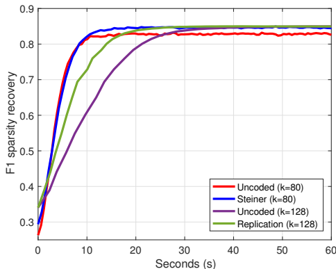
Figure 14: Evolution of F1 sparsity recovery performance for each scheme.
