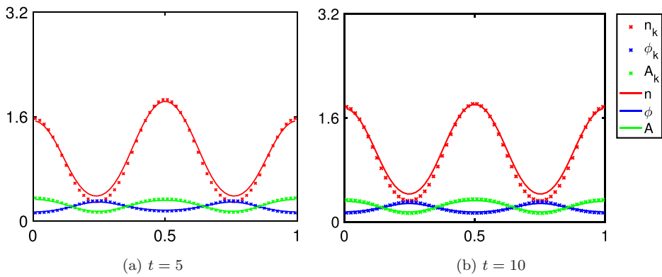
Fig. 8. Comparisons of the discrete and the continuum models with a BRW deployment strategy. All the parameters and data are the same as in Fig. 7. The system enters a steady state roughly at t = 10 .
