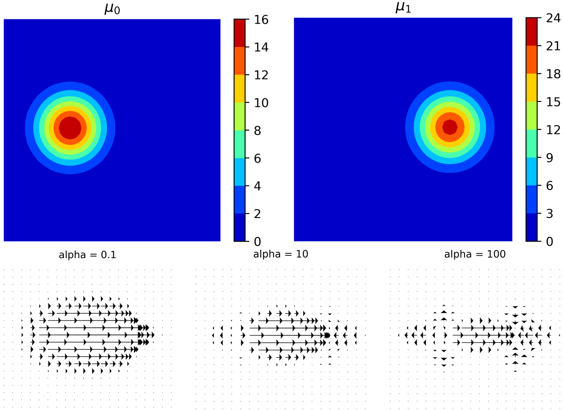
FIGURE 8. Experiment 5. L^1 unnormalized optimal transportation with f(t, x) using different \alpha values.
