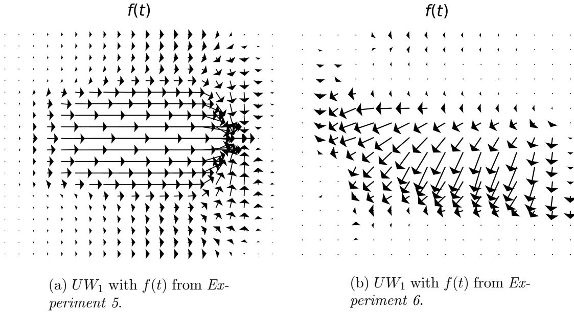
FIGURE 10. L^1 unnormalized optimal transportation with a spatially independent source function f(t) .
