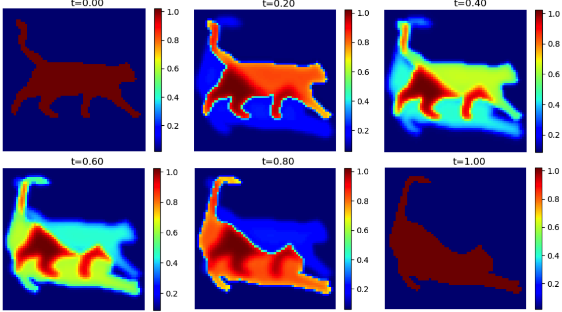
FIGURE 7. Experiment 4. L^2 generalized unnormalized optimal transportation: two cats example with a spatially dependent source function f(t, x) and \alpha = 1000 .
