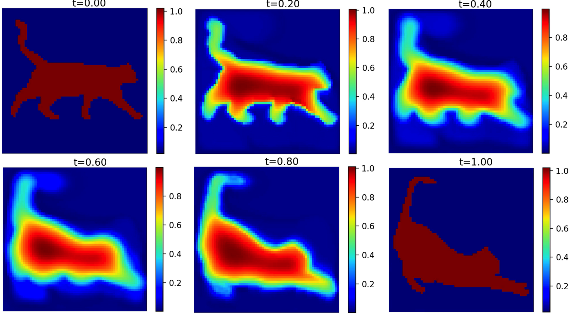
FIGURE 6. Experiment 4. L^2 generalized unnormalized optimal transportation: Two cats example with a spatially dependent source function f(t, x) and \alpha = 0.5 .
