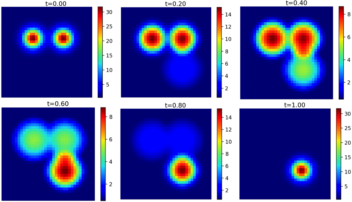
FIGURE 5. Experiment 3. L^2 generalized unnormalized optimal transportation: 2D example with a spatially dependent source function f(t, x) and \alpha = 1000 .
