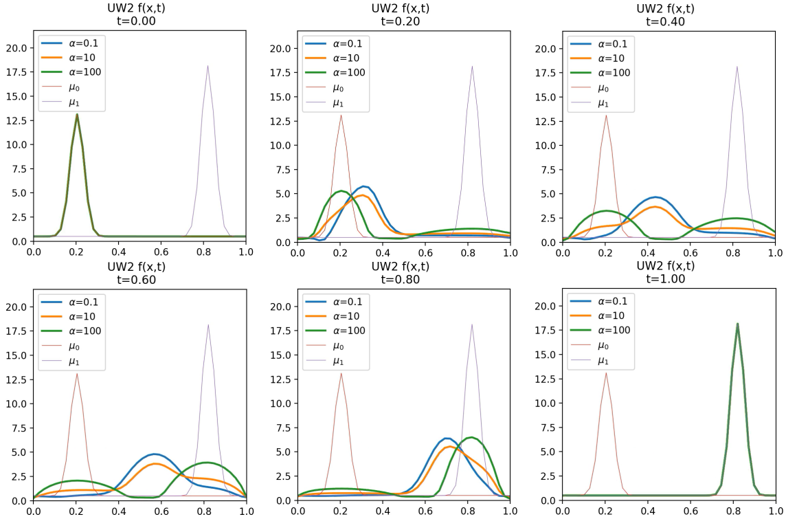
FIGURE 1. Experiment 1. L^2 Unnormalized optimal transportation with f(t, x) using different \alpha values. Blue line shows \alpha = 0.1 , orange line shows \alpha = 10 , and green line shows \alpha = 100 .
