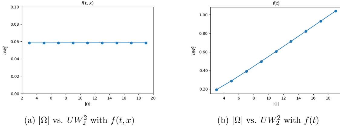
FIGURE 3. Experiment 2. The size of the domain |\Omega| vs. L^2 unnormalized Wasserstein metrics for f(t, x) and f(t) . x-axis represents |\Omega| and y-axis represents UW_2(\mu_0, \mu_1)^2 . Both f(t, x) and f(t) use \alpha = 100 .
