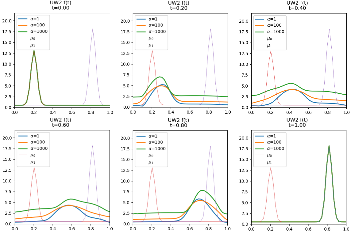
FIGURE 2. Experiment 1. L^2 Unnormalized optimal transportation with f(t) using different \alpha values. Blue lines show \alpha = 1 , orange lines show \alpha = 100 , and green lines show \alpha = 1000 .
