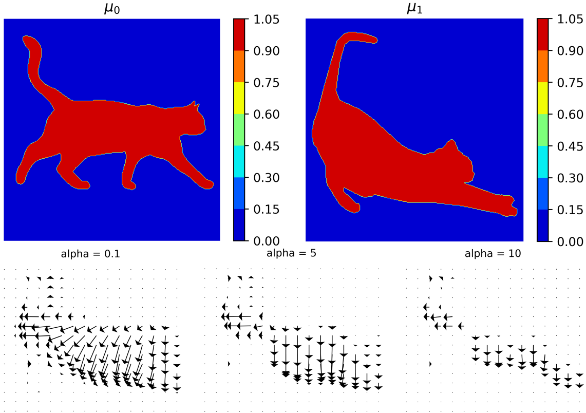
FIGURE 9. Experiment 6. L^1 unnormalized optimal transportation with f(t, x) using different \alpha values.
