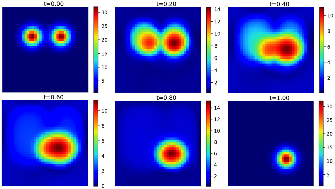
FIGURE 4. Experiment 3. L^2 generalized unnormalized optimal transportation: 2D example with a spatially dependent source function f(t, x) and \alpha = 1 .
