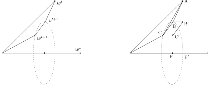
Fig. 2. Geometry of the update of \mathbf{w}^t and the corresponding \mathbf{w}^{t+1}, \mathbf{v}^{t+1} .
