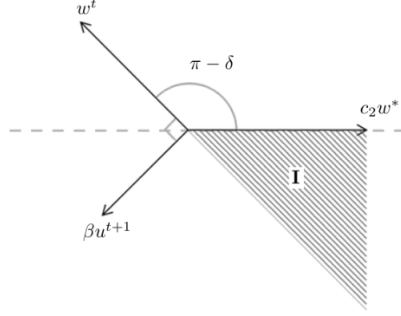
Fig. 3. Worst case of the update on w^t
