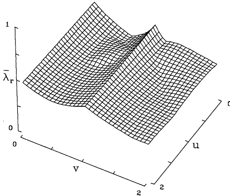
Fig. 2. Two-level convergence rate \bar{\lambda}_r as a function of u and v ( c = 1 ), for a 64 \times 64 grid with h_x = h_y , using damped Point-Jacobi smoothing with \nu_1 + \nu_2 = 1 , \nu_p = 0 . The worst convergence factor is \frac{1}{2} , for v = 0 and |u| = c .
