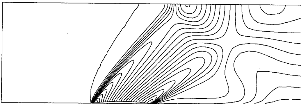
Fig. 4c. Iso-Mach lines for mach 0.85 inflow. Contours are 0.025 apart (first-order Osher scheme).
