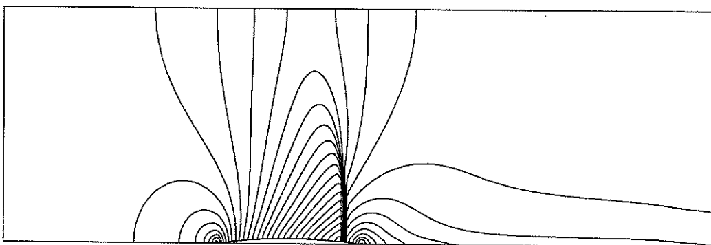
Fig. 4b. Iso-Mach lines for mach 0.5 inflow. Contours are 0.01 apart (first-order Osher scheme). The asymmetry gives an indication of the low accuracy of the first-order scheme.
