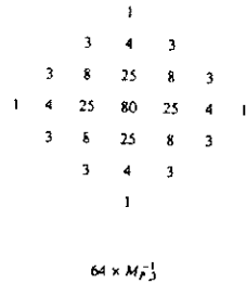
Fig. 5. Stencil representation of the local operator for the polynomial preconditioner.
