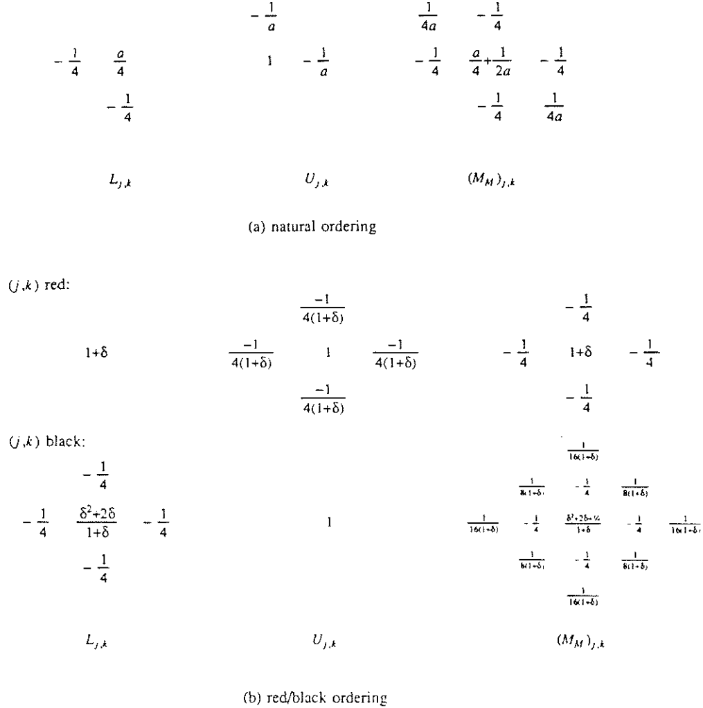
Fig. 4. Stencil representations of local operators for the MILU preconditioner.
