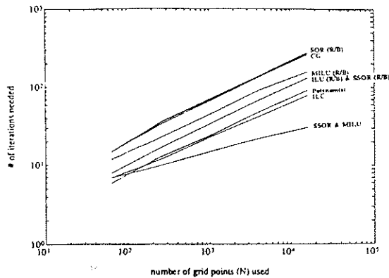
Fig. 6. Convergence rates for SOR (R/B) and PCG methods.
