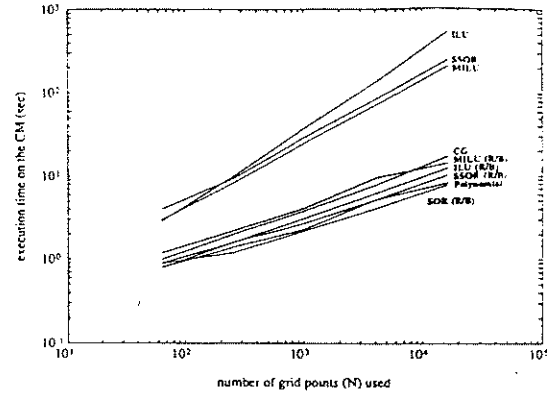
Fig. 7. CM execution time for SOR(R/B) and PCG methods.
