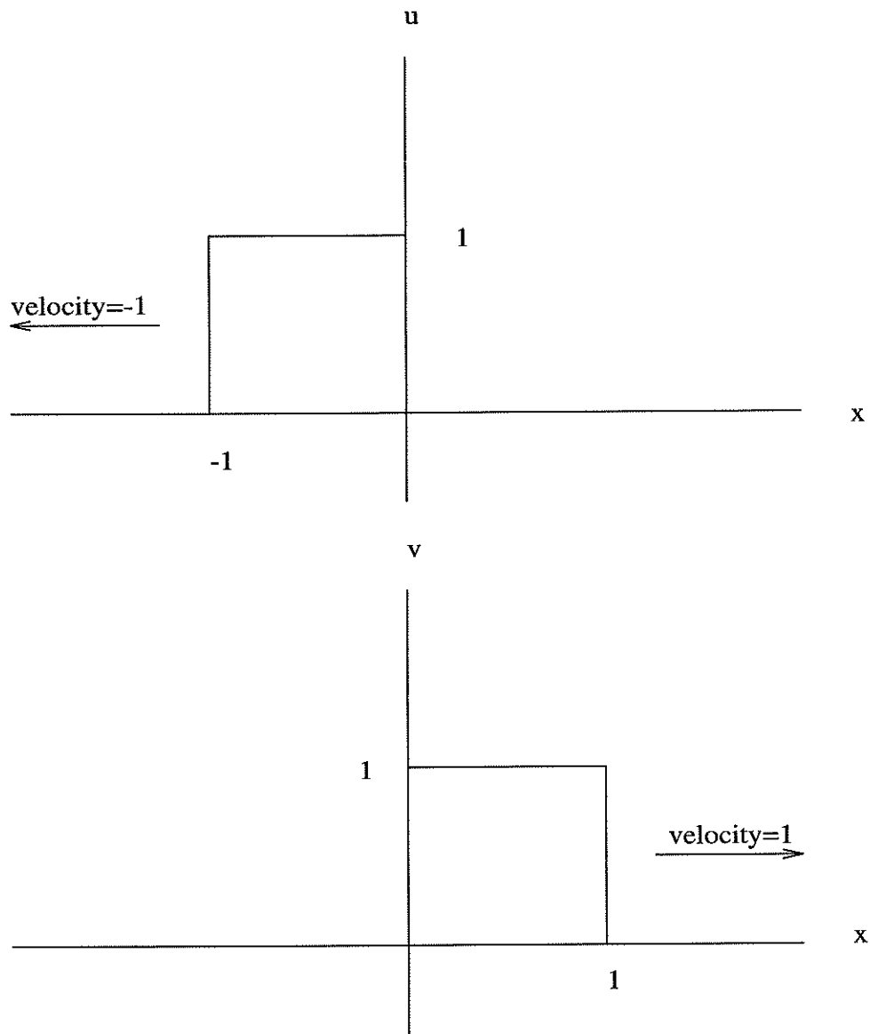
Figure 1: Initial data for the two independent wave equations, resulting in simple translation to the left and to the right.
