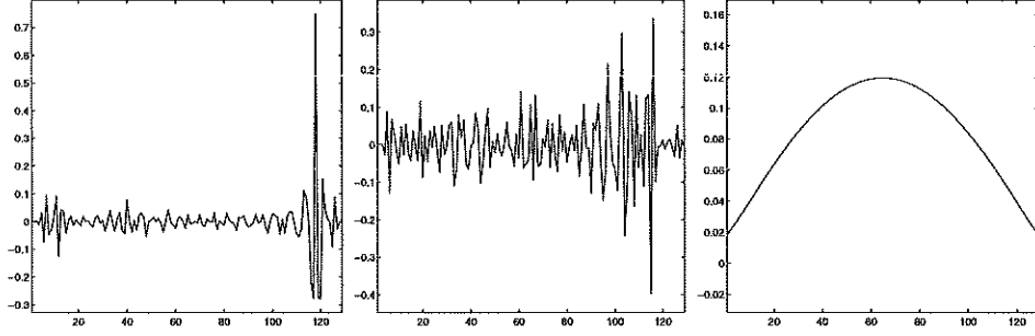
Fig. 1. Eigenvectors corresponding to (a) the smallest (b) the middle (c) the largest eigenvalue of L = 10^{-4}I + K . The oscillatory eigenvectors corresponding to the small eigenvalues.
