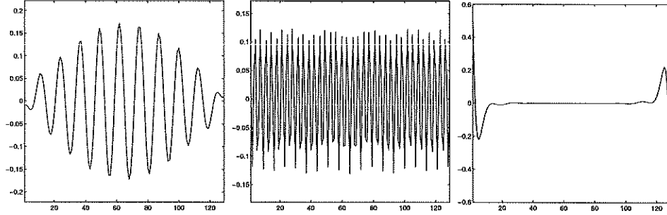
Fig. 7. Eigenvectors corresponding to (a) the smallest (b) the middle (c) the largest eigenvalue of the cosine transform preconditioned system of L = 10^{-4}I + K . The oscillatory eigenvectors are clustered in the middle of the spectrum.
