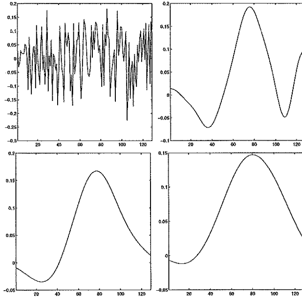
Fig. 5. Error vectors after 0 iteration (top left), 1 iteration (top right), 5 iterations (bottom left) and 10 iterations (bottom right) of Richardson smoothing applied to L = I - K . The oscillatory components are quickly smoothed out.
