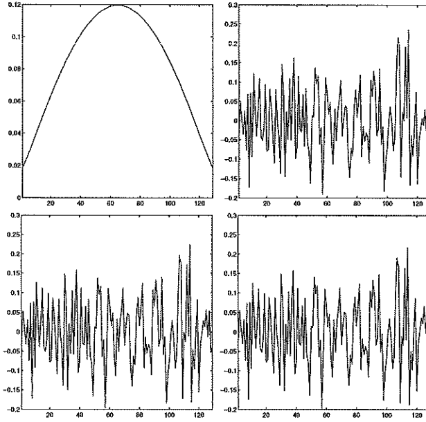
Fig. 3. Error vectors after 0 iteration (top left), 1 iteration (top right), 5 iterations (bottom left) and 10 iterations (bottom right) of Richardson smoothing applied to L = 10^{-4}I + K . The smooth component is removed completely after only 1 iteration whereas the oscillatory components persist. All the plots are scaled so that the l_2 -norm of the vector is equal to 1.
