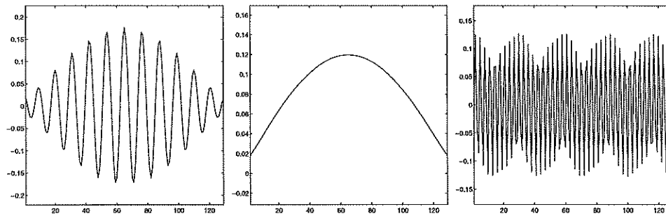
Fig. 11. Eigenvectors corresponding to (a) the smallest (b) the middle (c) the largest eigenvalue of L = -10^{-8}\Delta + K . When \alpha is small, the eigenvectors of L resemble those of K .
