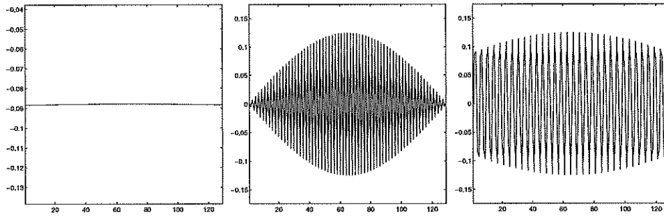
Fig. 9. Eigenvectors corresponding to (a) the smallest (b) the middle (c) the largest eigenvalue of L = -\Delta + K . When \alpha is large, the eigenvectors of L resemble those of -\Delta .
