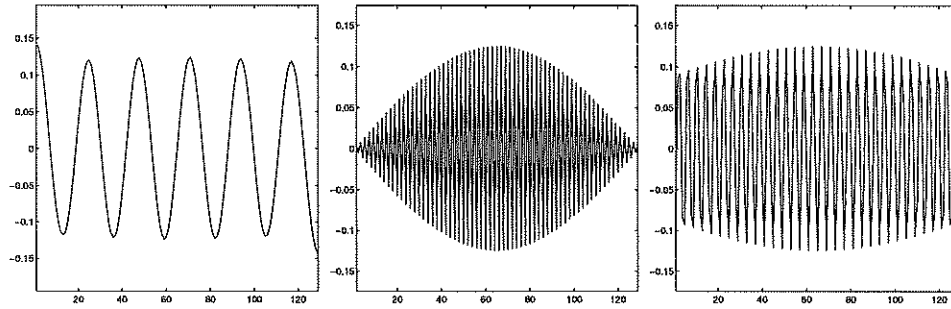
Fig. 10. Eigenvectors corresponding to (a) the smallest (b) the middle (c) the largest eigenvalue of L = -10^{-4}\Delta + K . For intermediate value of \alpha , the eigenvectors corresponding to large eigenvalues resemble those of -\Delta and the eigenvectors corresponding to small eigenvalues are oscillatory and resemble those of K .
