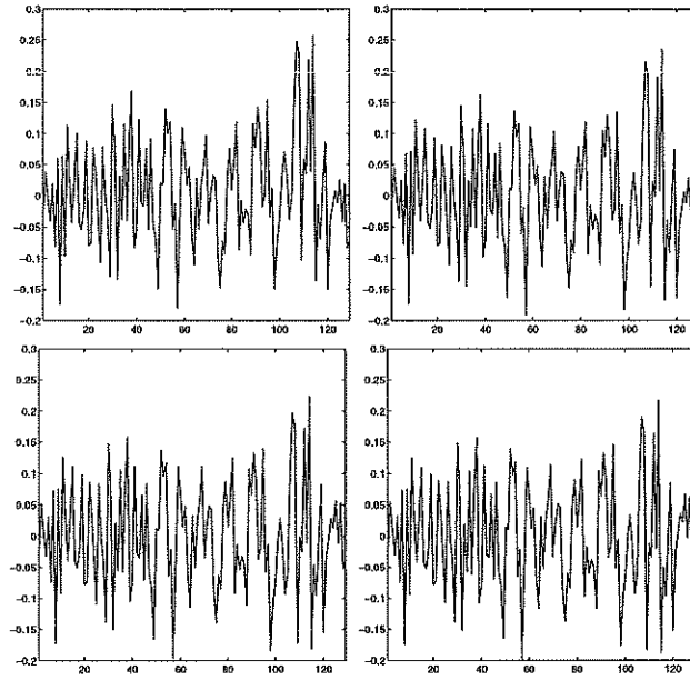
Fig. 2. Error vectors after 0 iteration (top left), 1 iteration (top right), 5 iterations (bottom left) and 10 iterations (bottom right) of Richardson smoothing applied to L = 10^{-4}I + K . Note that there is no smoothing effect.
