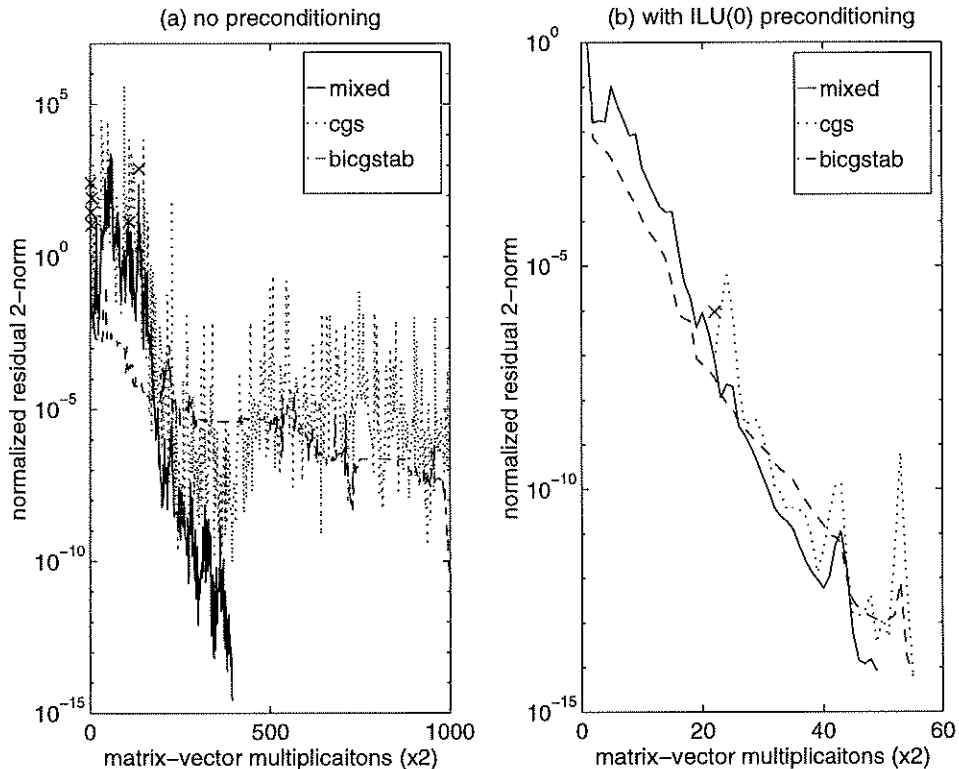
FIG. 3. Convergence History for Example 3
