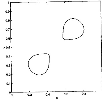
(c) t = 0.02
