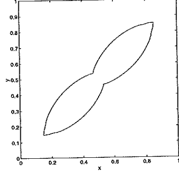
(b) A Gaussian kernel. In this example, K = K_G^{\Delta t^2} .
