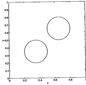
(a) t = 0.0000
