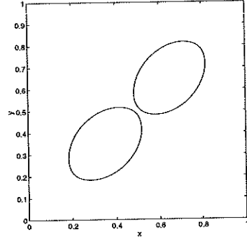
(b) t = 0.0333
