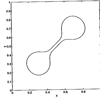
(b) t = 0.01
