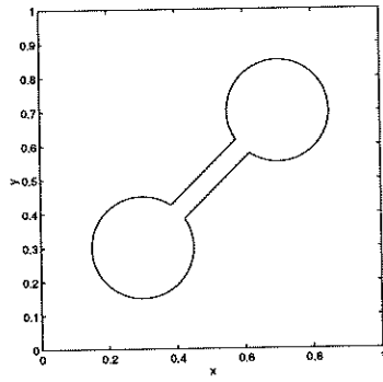
(a) t = 0.00
