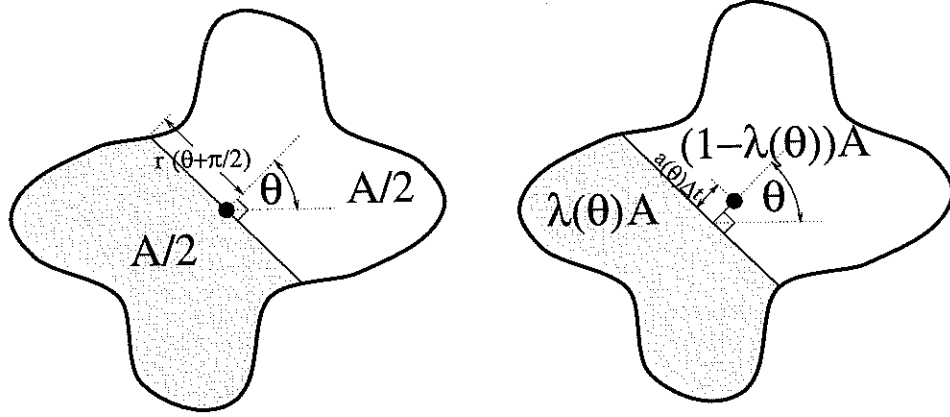
(b) For general anisotropic motions \lambda(\cdot) depends on \theta .
