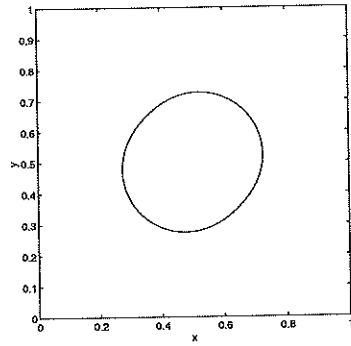
(c) t = 0.0333
