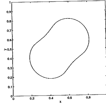
(b) t = 0.0167
