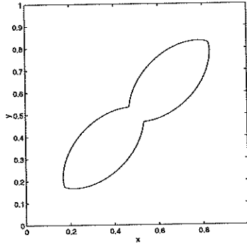
(c) t = 0.0667
