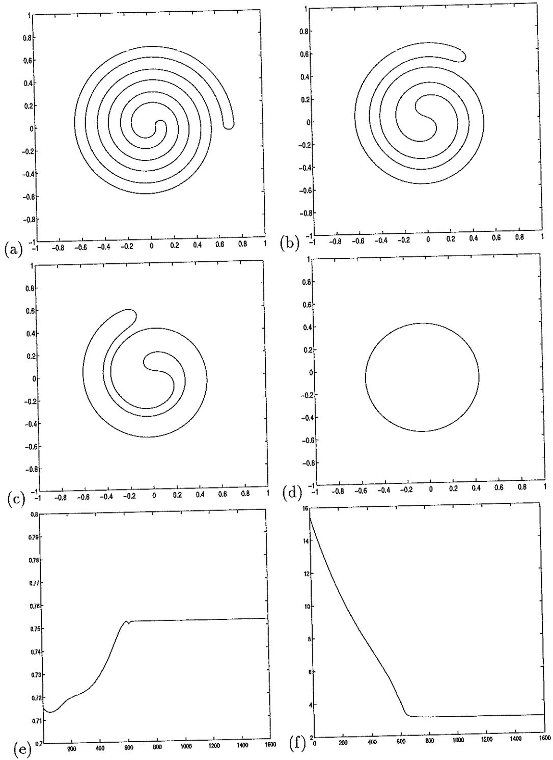
Figure 9: Volume conserved mean curvature flow. Grid 128 \times 128 , RK3-WENO5. (a) Initial front. (b) After 200 steps. (c) After 400 steps. (d) After 1600 steps. (e) Area. (f) Arclength.
