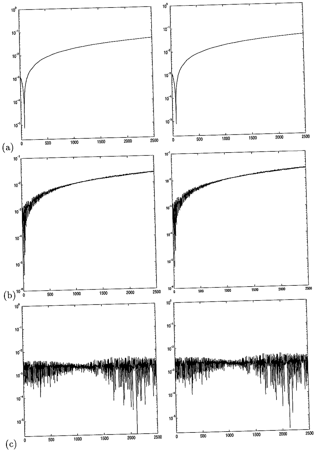
Figure 8: Data on the left are computed with global method, while the right are computed with local method. Grid 128 \times 128 . RK3-ENO3. (a) Percentage of area loss. (b) Percentage of arclength loss. (c) Deviation from 1 of defect ratio.
