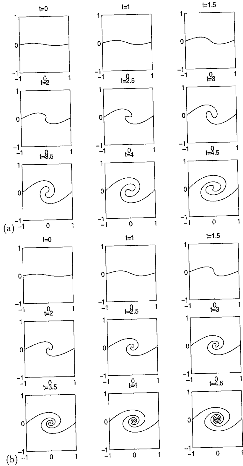
Figure 11: Vortex sheet problem. \Delta t = 0.1\Delta x . (a) Without reinitialization and extension. (b) With reinitialization and extension every 10 time step.
