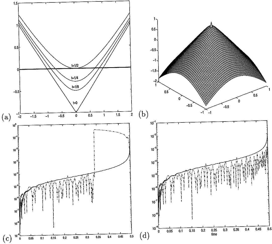
Figure 5: (a) The mid-slice of analytical level set function of a shrinking circle. (b) A spike appears at the center with a direct implementation. (c) The plot of errors in radius computed with reinitialization (solid line) and without reinitialization and without enforcing the internal boundary condition (28) (dashed line). Note that at about t = 0.35 , a spurious circle appear at the center. In this case, the radius is taken as the average of the two. (d) The plot of errors in radius computed with reinitialization (solid line) and without reinitialization and with enforcing the internal boundary condition (28) (dashed line).
