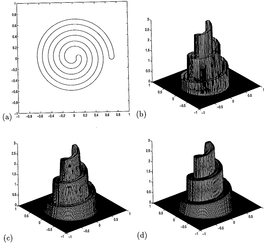
Figure 4: Extension. (a) Zero contour of \phi . (b) Initial q . (c) Extend for 5 steps. (d) Extend for 10 steps.
