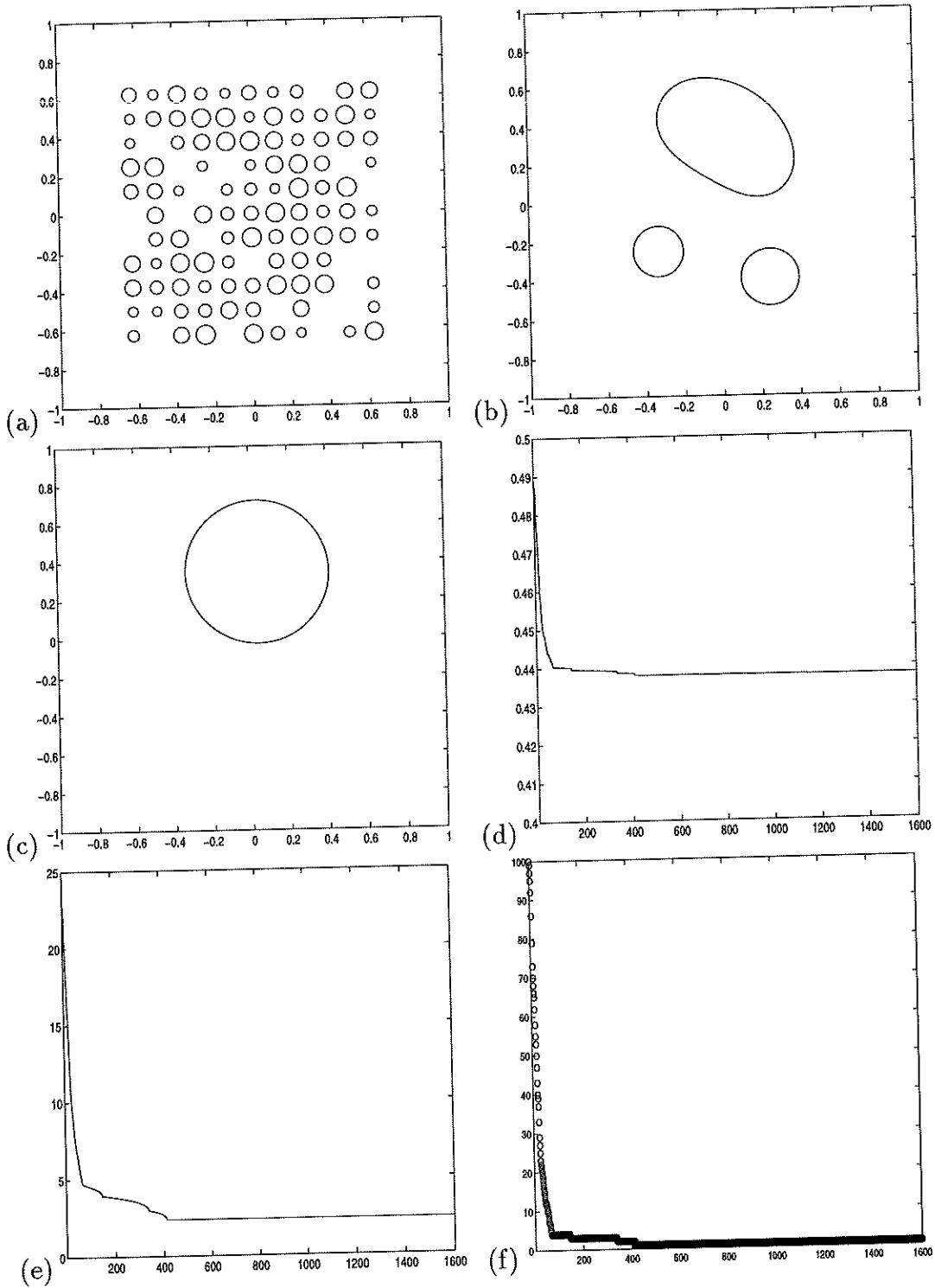
Figure 10: Volume conserved mean curvature flow. Grid 128 \times 128 , RK3-WENO5. (a) Initial fronts. (b) After 200 steps. (c) After 1600 steps. (d) Area. The exact area is 0.4613. (e) Arclength. The initial arclength is 23.598. (f) Number of bubbles. The initial number of bubbles is 100.
