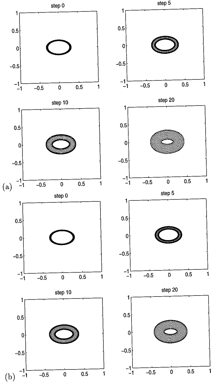
Figure 7: For a steep \phi , the interface is moved substantially with the approximation to S(\phi) as (30), while the new one given by (36) alleviates the problem quite a bit. The initial level \phi(x, y) = x^2/.3^2 + y^2/.2^2 - 1 , and the grid is 128 \times 128 , \Delta t = .5\Delta x . RK3-ENO3 is used. The contour is taken over [-10\Delta x : 2\Delta x : 10\Delta x] . (a) Approximate S(\phi) by \phi/\sqrt{\phi^2 + \Delta x^2} . (b) Approximate S(\phi) by \phi/\sqrt{\phi^2 + (|\nabla\phi|\Delta x)^2} .
