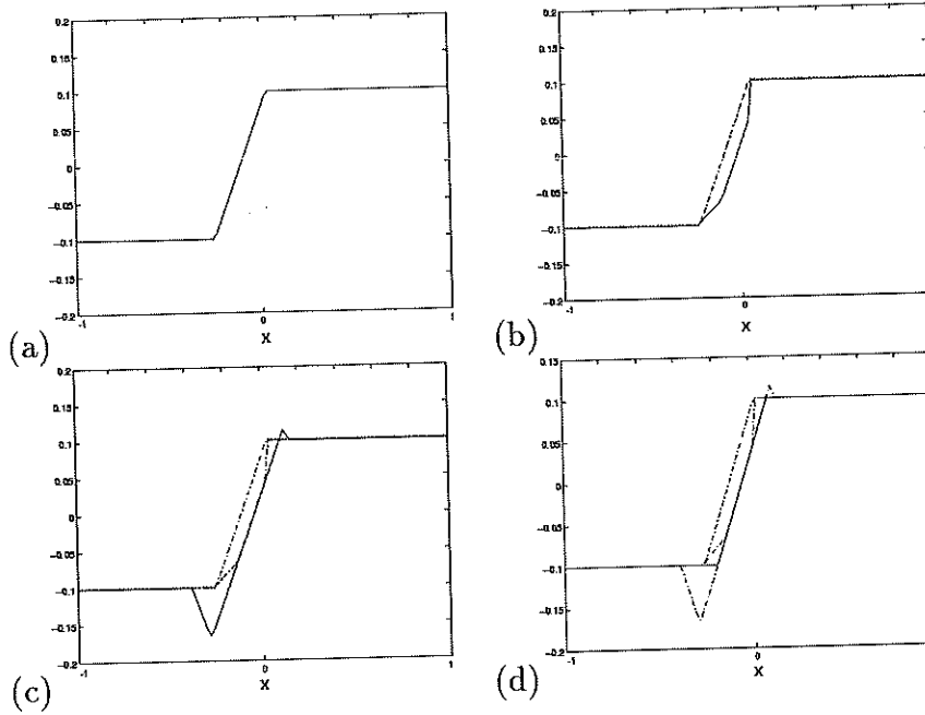
Figure 3: The current result is plotted with solid line, while the previous result(s) is shown with dashed line. (a) The initial local level set profile. (b) After moving one step. Note the steep gradient developing at the right tube boundary. (c) After reinitialization. (d) The final local level set profile after cutoff.
