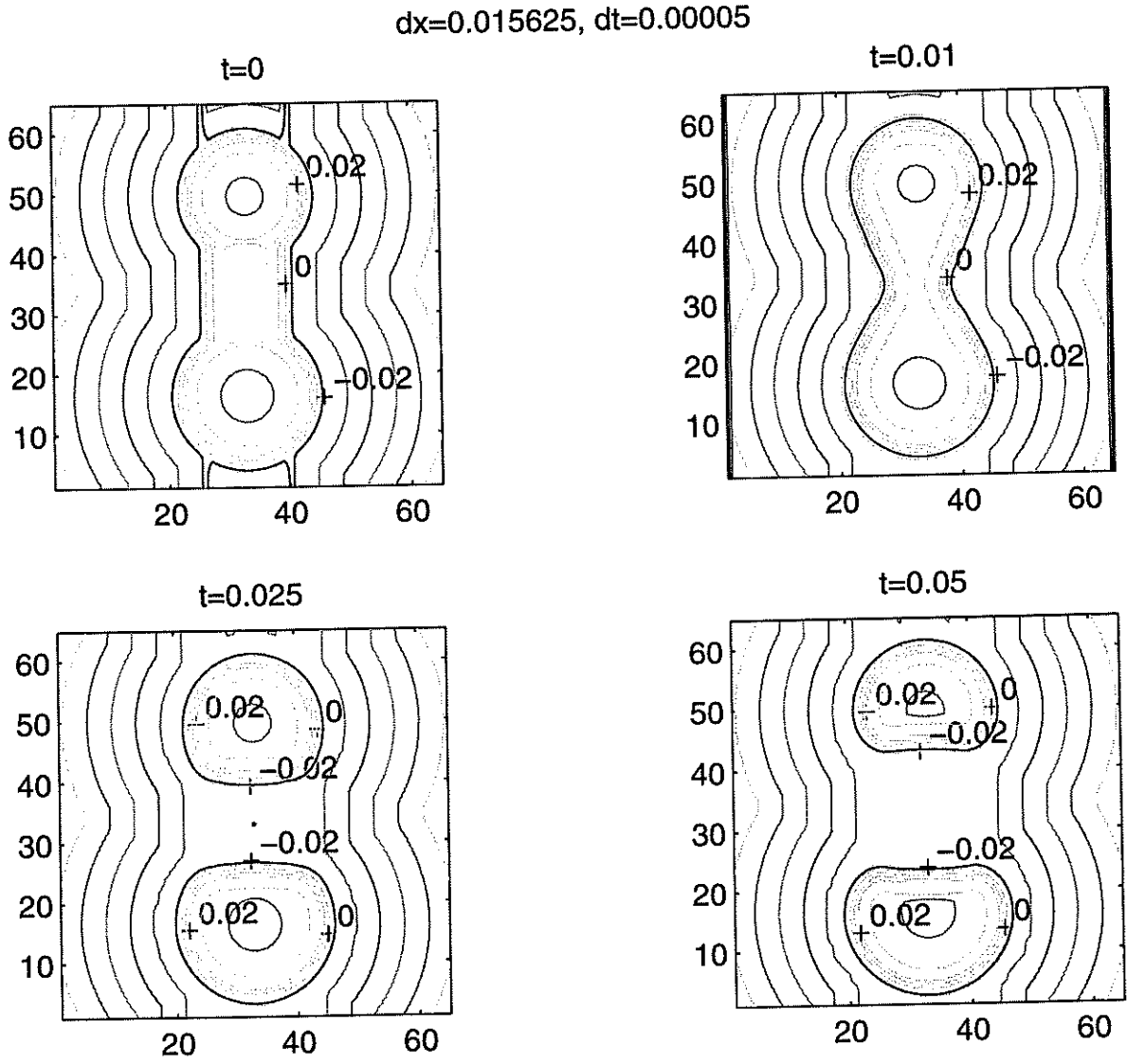
Figure 14: Middle slice of the 3D double bubble minimizer problem. The surface tension of the dumbbell is smaller than that of doughnut.
