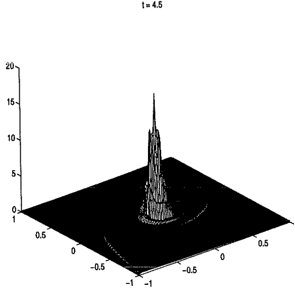
Figure 12: Vortex sheet problem. The vorticity at time t = 4.5 .
