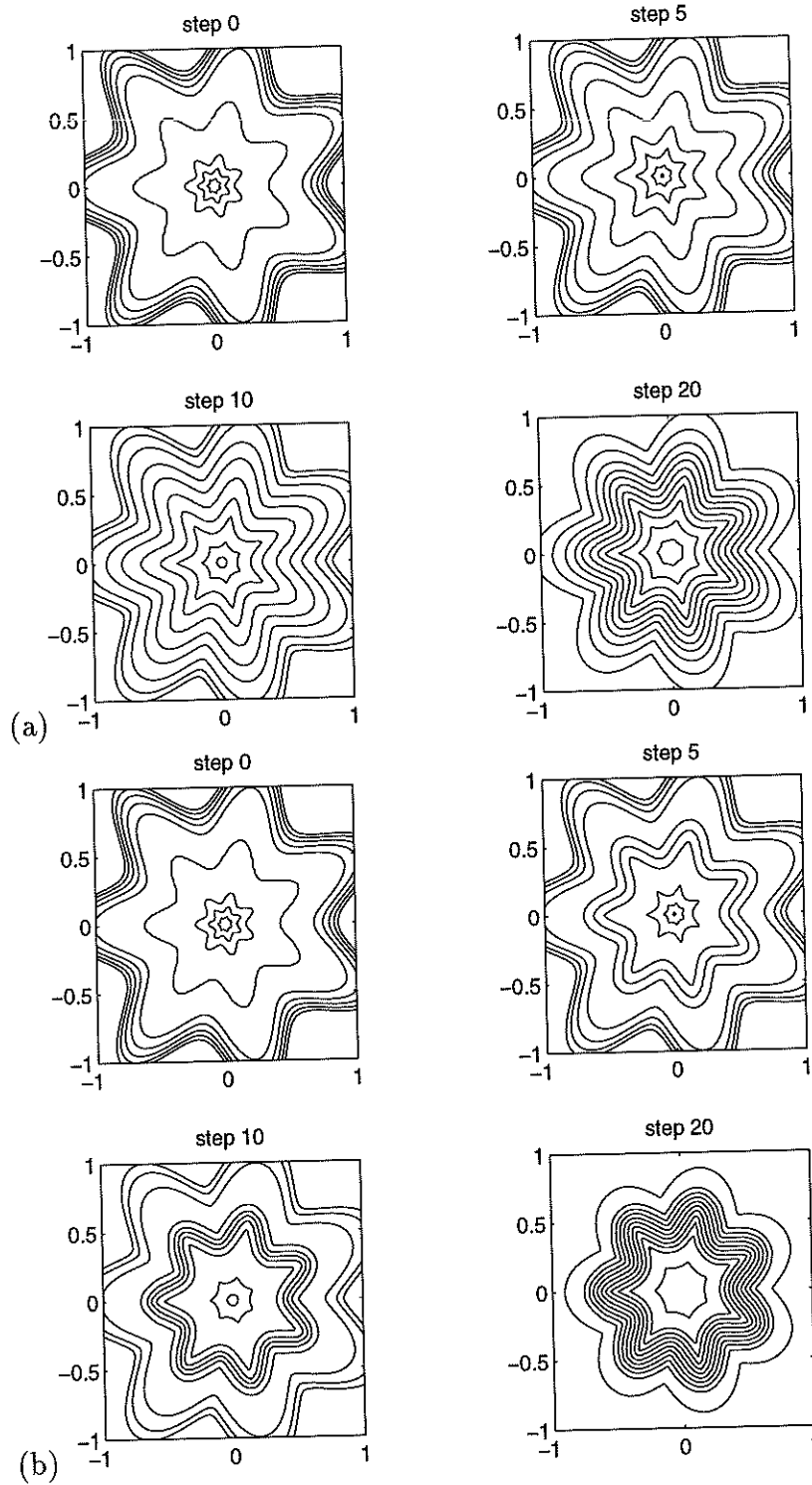
Figure 6: Convergence rate comparison for a flat \phi with different approximation to S(\phi) . The initial level set in polar coordinates is \phi(r, \theta) = (r - 0.5 + 0.1r \sin(7\theta))^3 . Grid 128 \times 128 , \Delta t = .5\Delta x . RK3-ENO3. Contour taken over [-10\Delta x : 2\Delta x : 10\Delta x] . (a) Approximate S(\phi) by \phi/\sqrt{\phi^2 + \Delta x^2} . (b) Approximate S(\phi) by \phi/\sqrt{\phi^2 + (|\nabla\phi|\Delta x)^2} .
