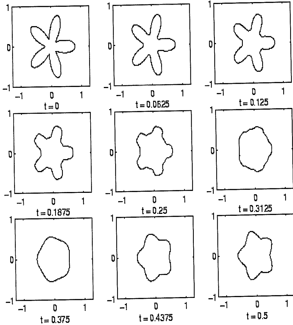
Figure 13: Oscillating starfish, curvature dependent acceleration(volume preserving). Initial shape is given in polar coordinate by r = 0.5 + 0.3 \sin 5\theta .
