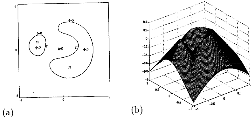
Figure 1: (a) Zero contour of \phi representing the front \Gamma . (b) Surface of -\phi .
