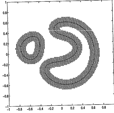
Figure 2: Computation is only performed on the marked region around \Gamma .
