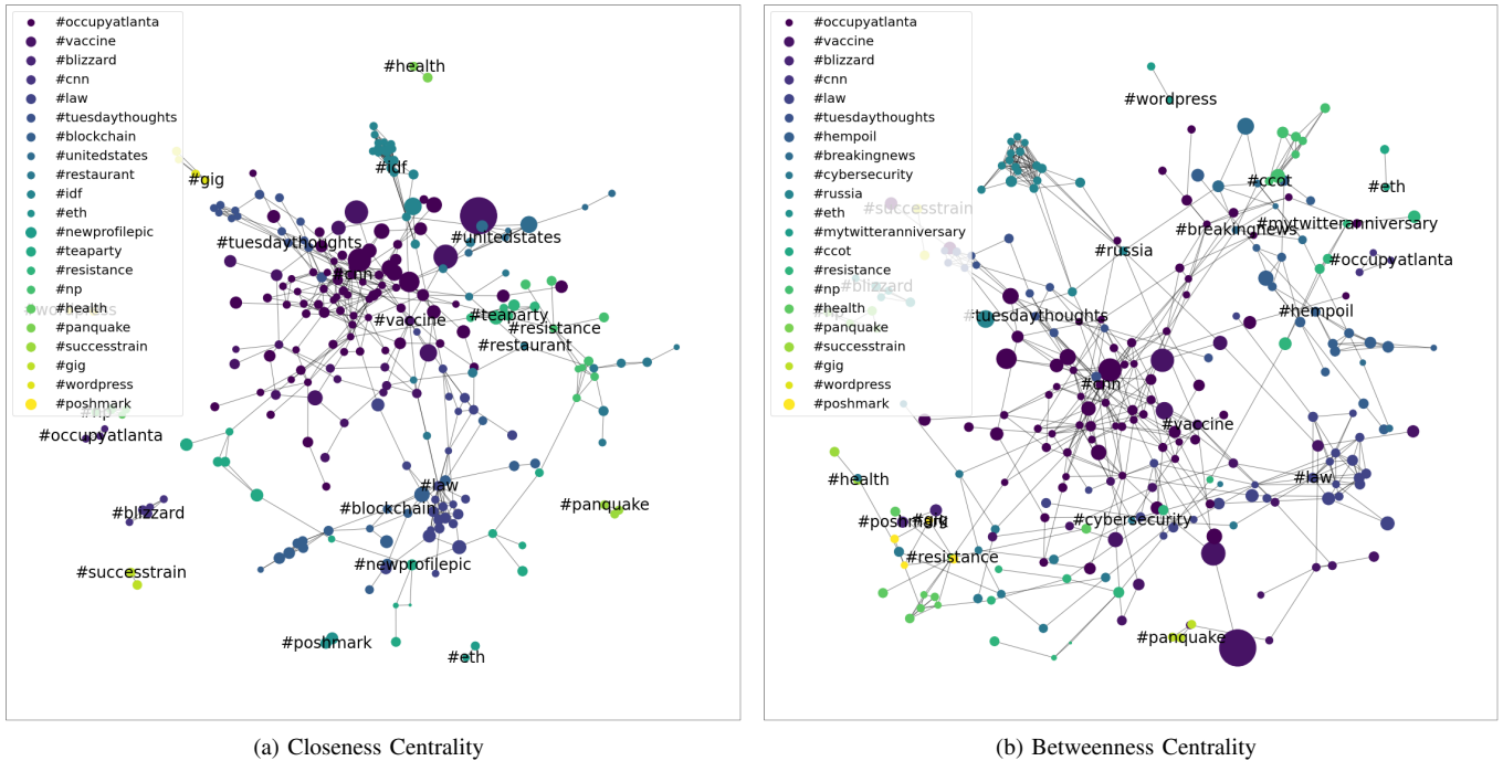
Fig. 2: (a) Hashtag co-occurrence graphs with communities labeled by highest closeness centrality, and (b) communities labeled by highest betweenness centrality. The node size indicates the frequencies of each hashtag, the edges represent the co-occurrence relations, and the colors distinguish between different communities.
