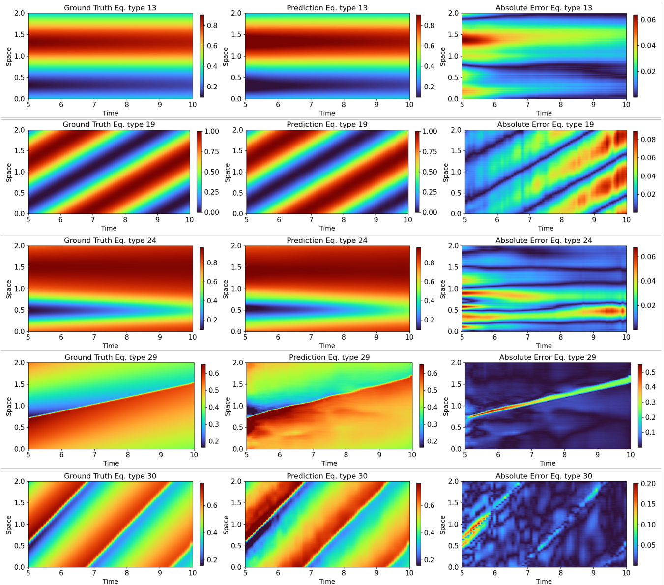
Figure 3: Example of extrapolation in time. The model is trained on data generated for t \in [0, 5] and tasked to predict the solution for t \in [5, 10] . From left to right, ground truth solution, predicted solution, absolute difference. First row: Heat Equation (index 13), Second row: Advection Equation (index 19). Third row: Diffusion-reaction Square Logistic (index 24). Fourth row: Inviscid Conservation law Cubic Flux (index 29) ; Fifth row: Conservation law Sine Flux (index 30)
